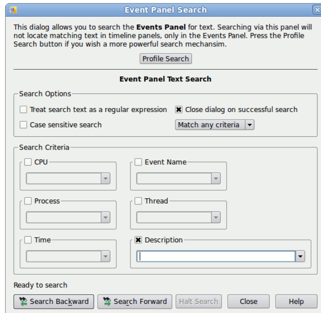
Figure 4-41. NightTrace - Event Panel Search Dialog
