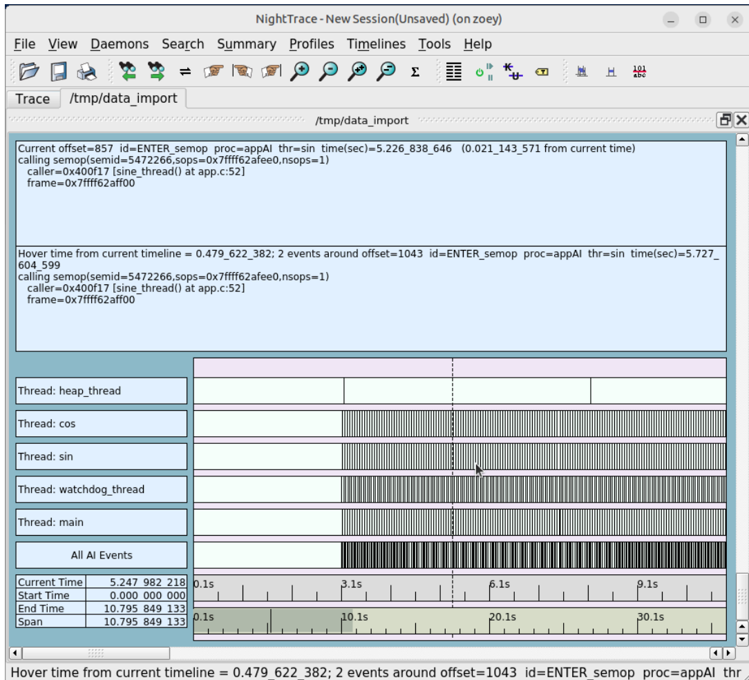
Figure 4-39. NightTrace - /tmp/data_import Timeline
