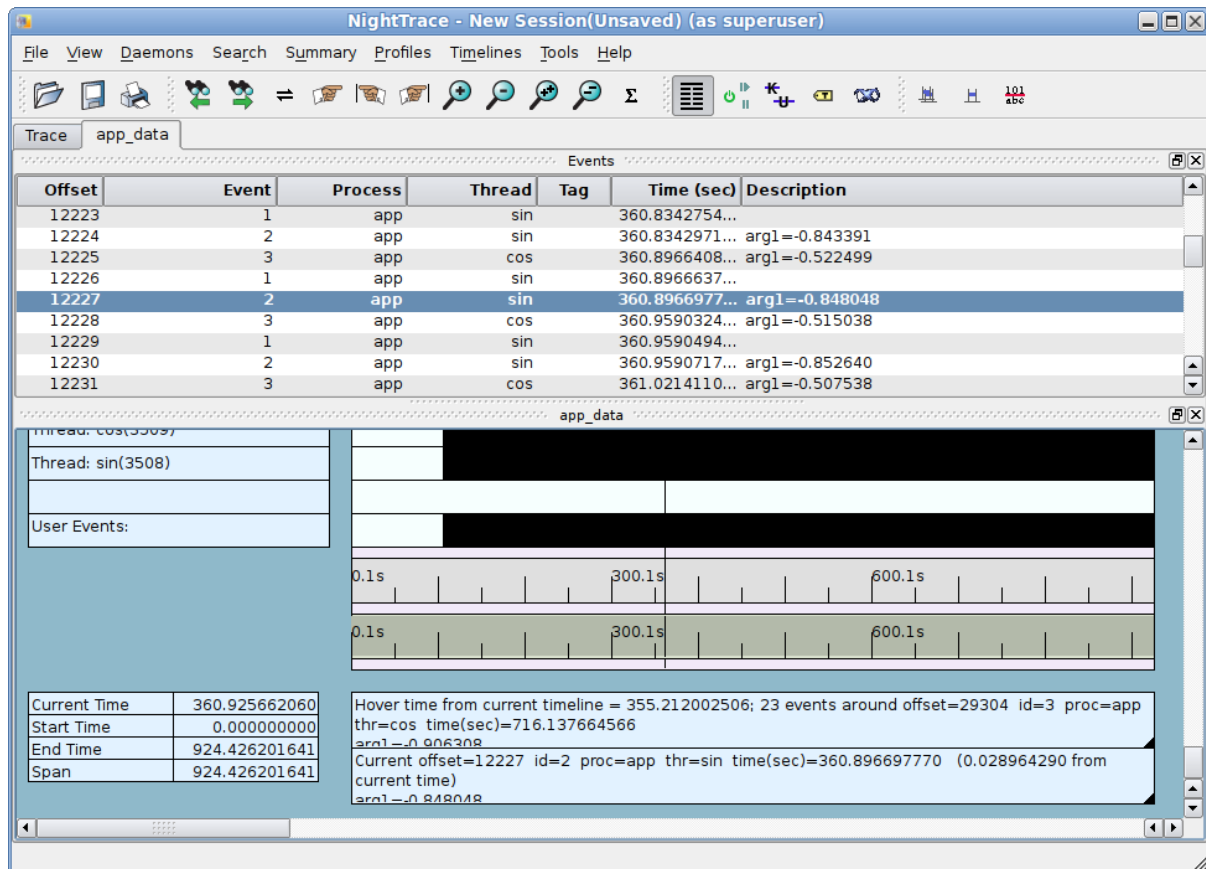
Figure 4-5. NightTrace Timeline
