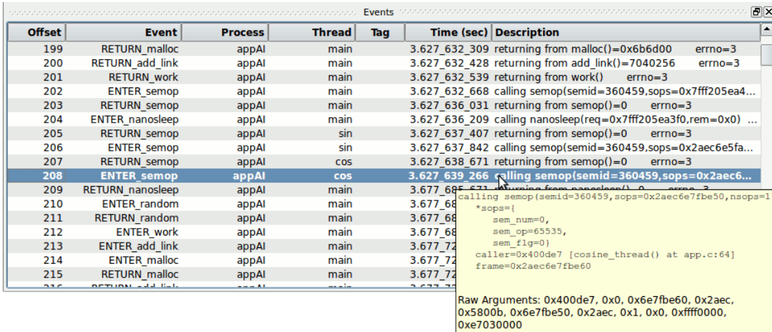
Figure 4-40. NightTrace - Events Panel w/ Tool Tip
