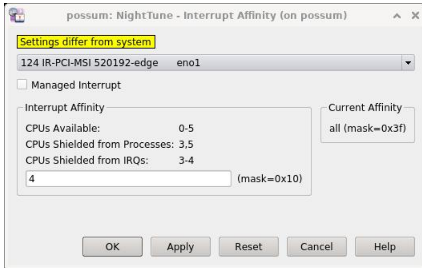
Figure 5-15. Interrupt Affinity Dialog
