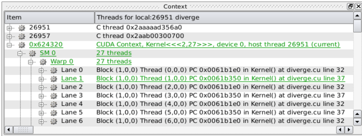
Figure 8-7. Threads Data Item with CUDA context and threads
