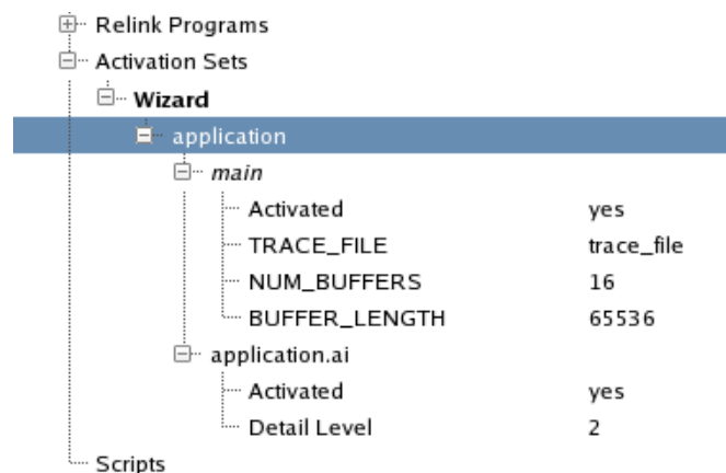
Figure 5-19. Activation Sets Advanced Settings
