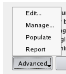
Figure 5-12. Advanced Menu
