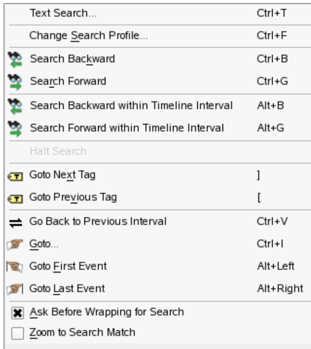
Figure 8-6. Search Menu
