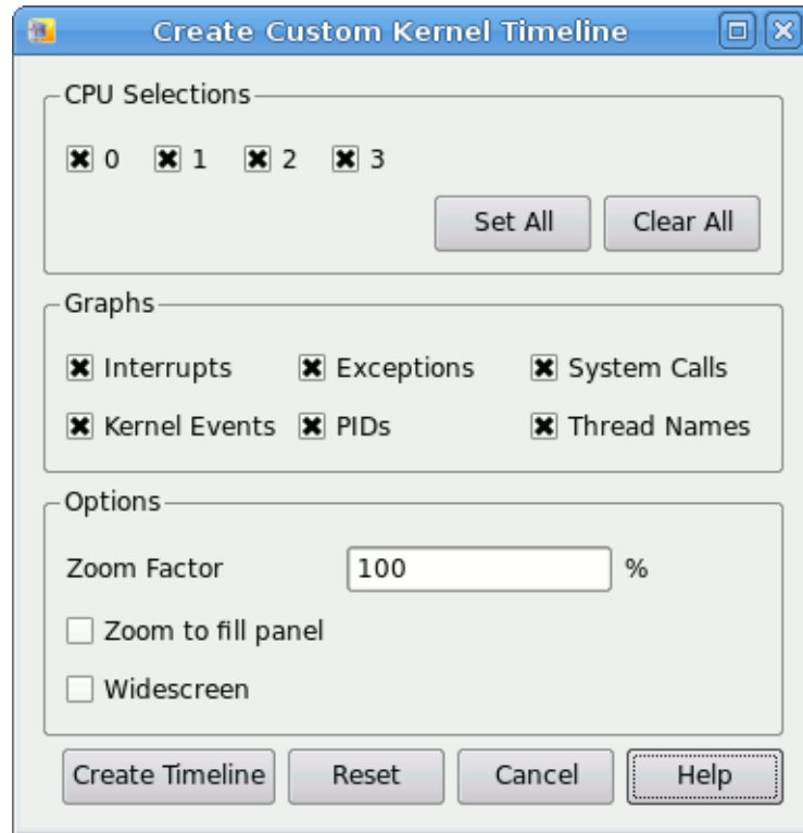
Figure 8-13. Create Custom Kernel Timeline Dialog
