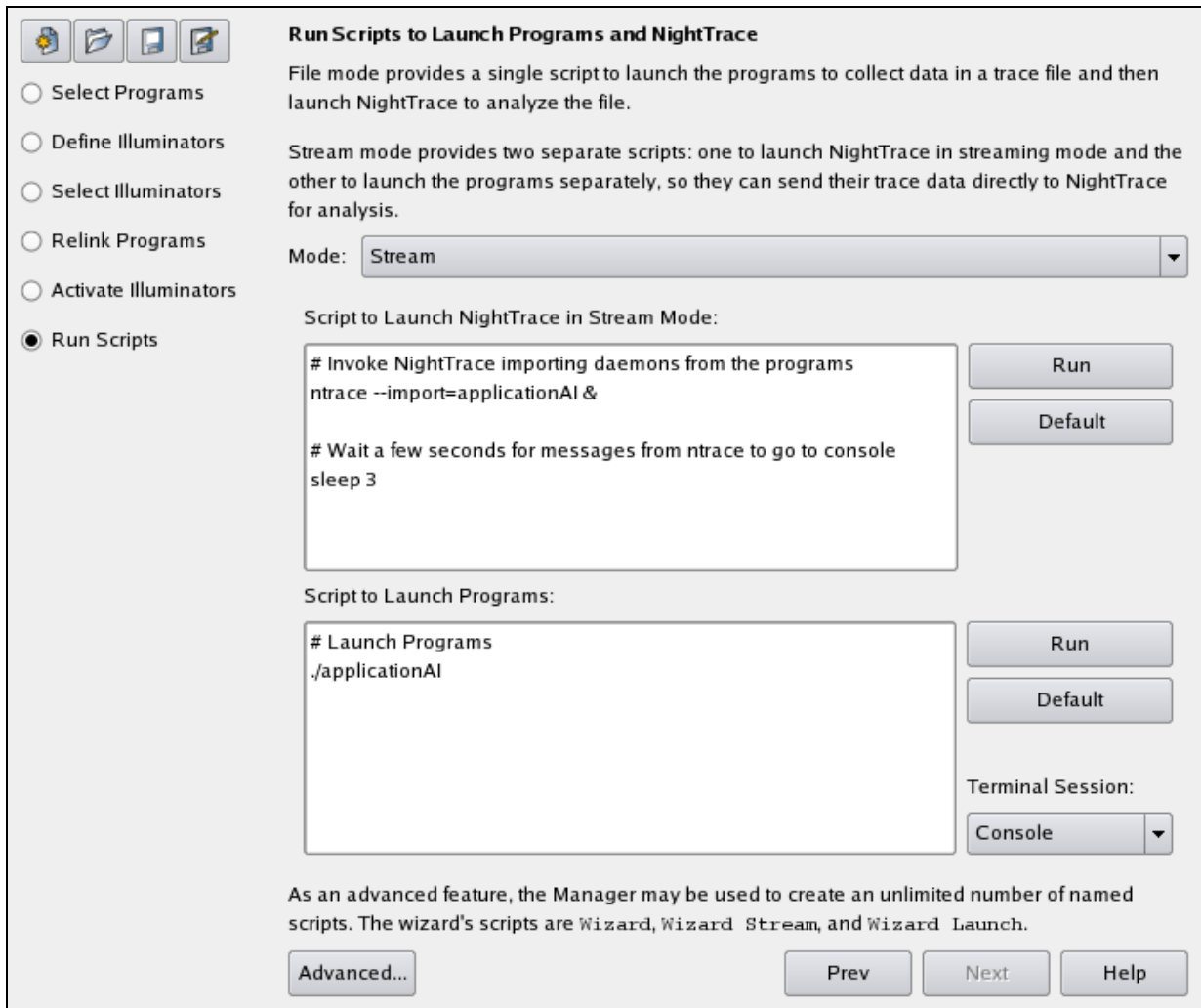
Figure 5-21. Run Scripts to Launch Programs and NightTrace Dialog in Stream Mode
