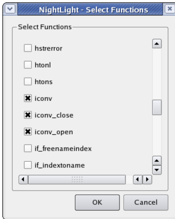
Figure 5-79. Select Functions Dialog
