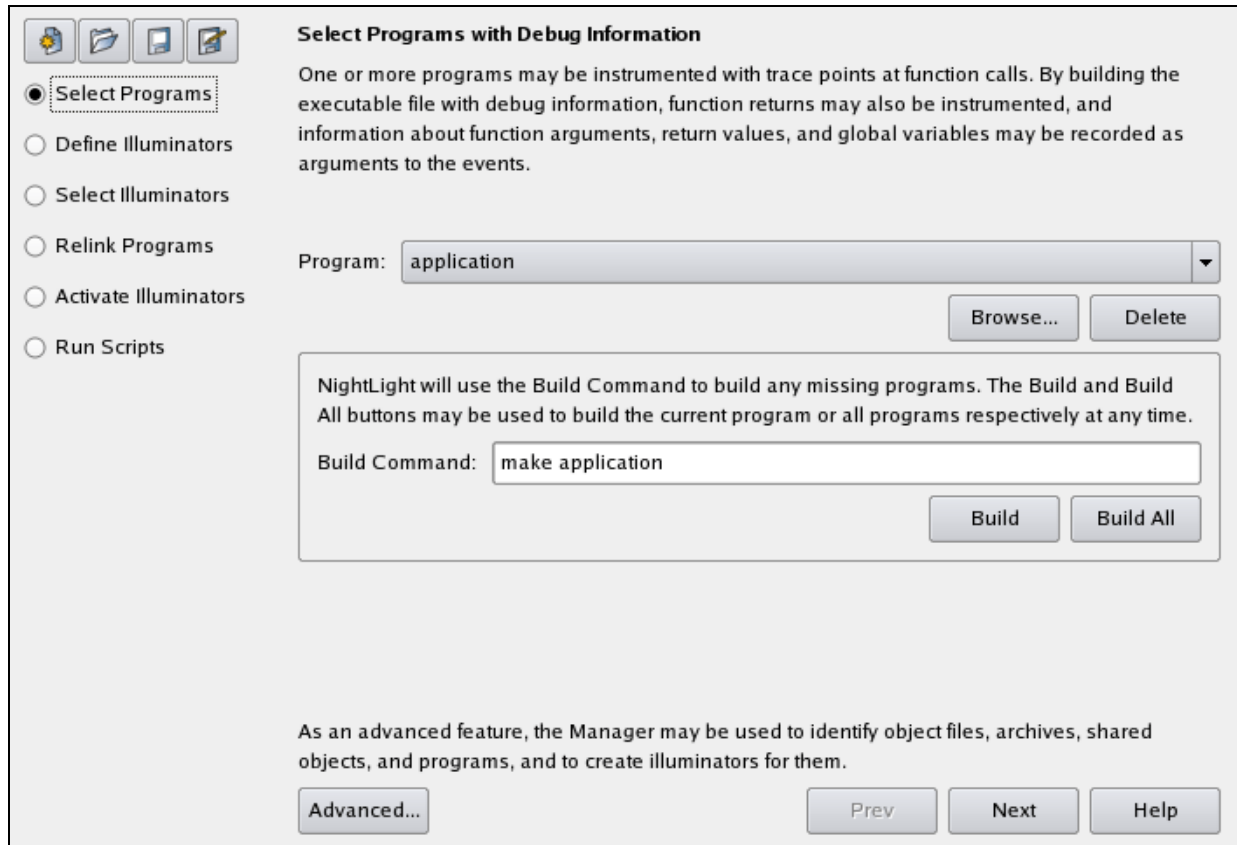
Figure 5-9. Select Programs with Debug Information Dialog
