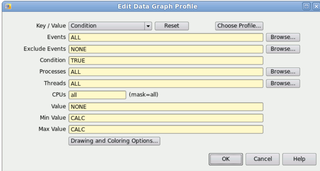
Figure 12-10. Edit Data Graph Profile Dialog
