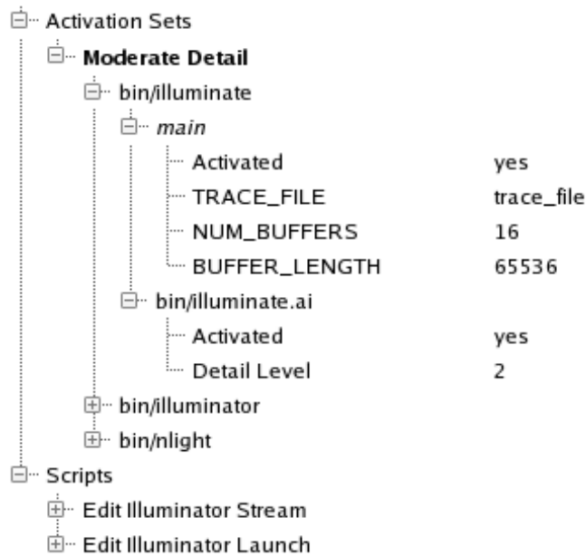
Figure 5-55. Activation Set for an Elaborate Script Example
