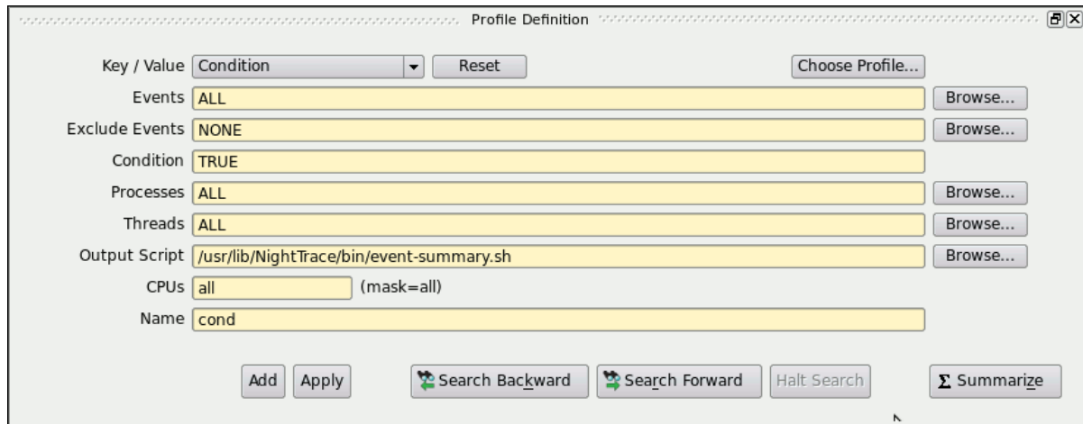
Figure 13-1. Profile Definition Panel
