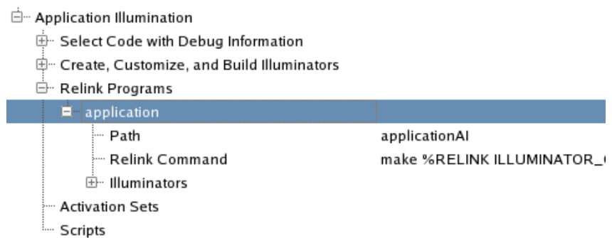
Figure 5-16. Relink Programs Advanced Settings
