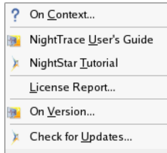
Figure 8-16. Help Menu
