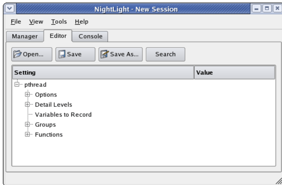
Figure 5-61. Editor Page
