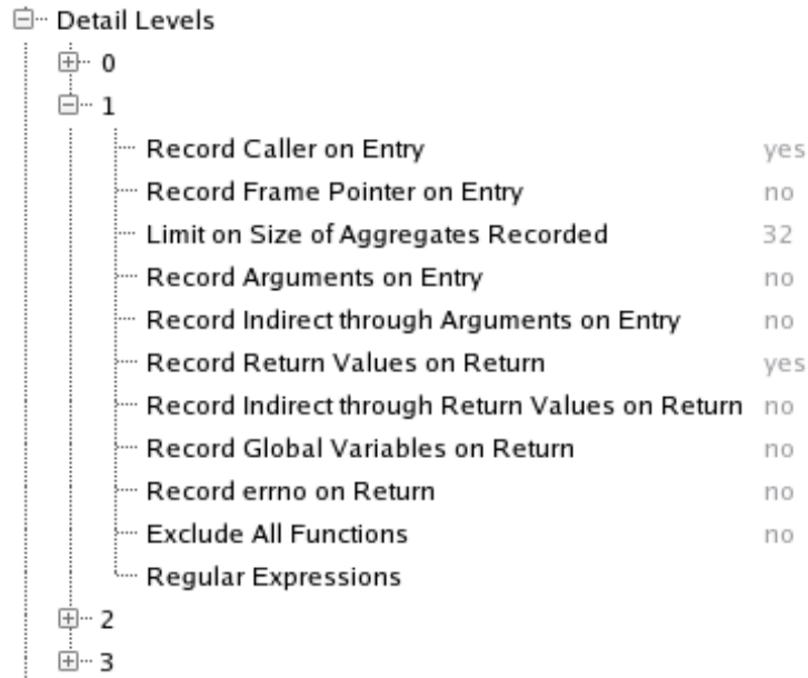
Figure 5-68. Detail Levels
