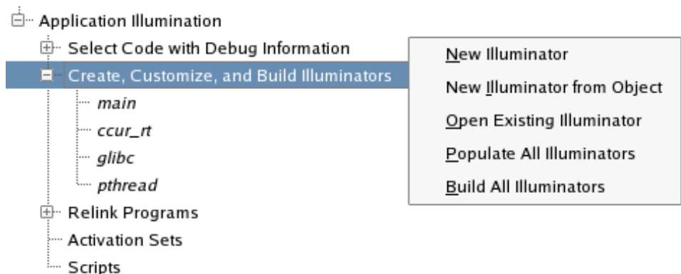
Figure 5-31. Create, Customize, and Build Illuminators Context Menu
