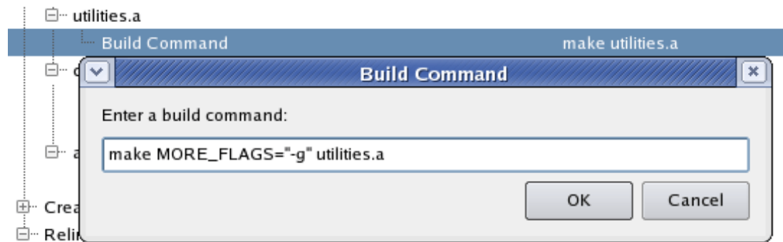
Figure 5-29. Build Command Dialog
