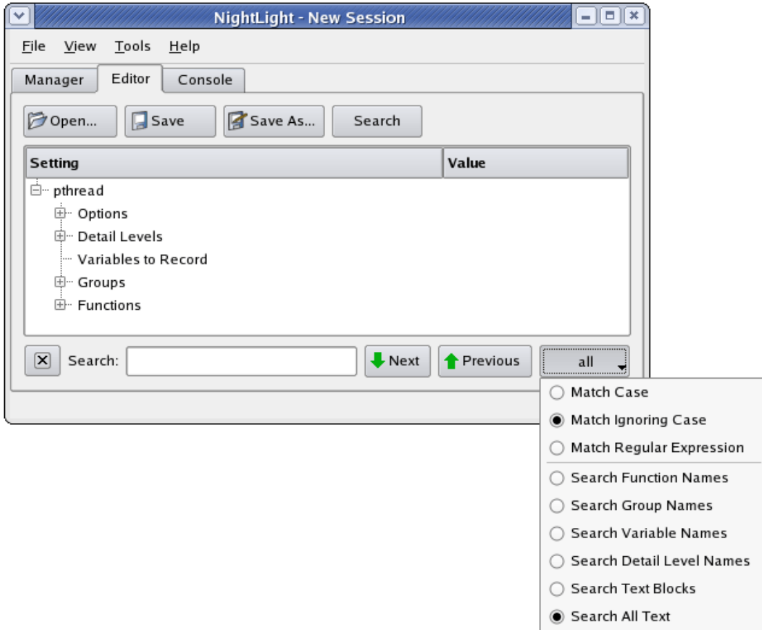
Figure 5-62. The Search Bar
