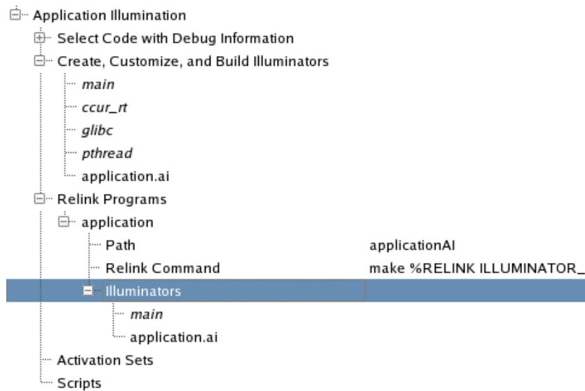
Figure 5-15. Select Illuminators Advanced Settings
