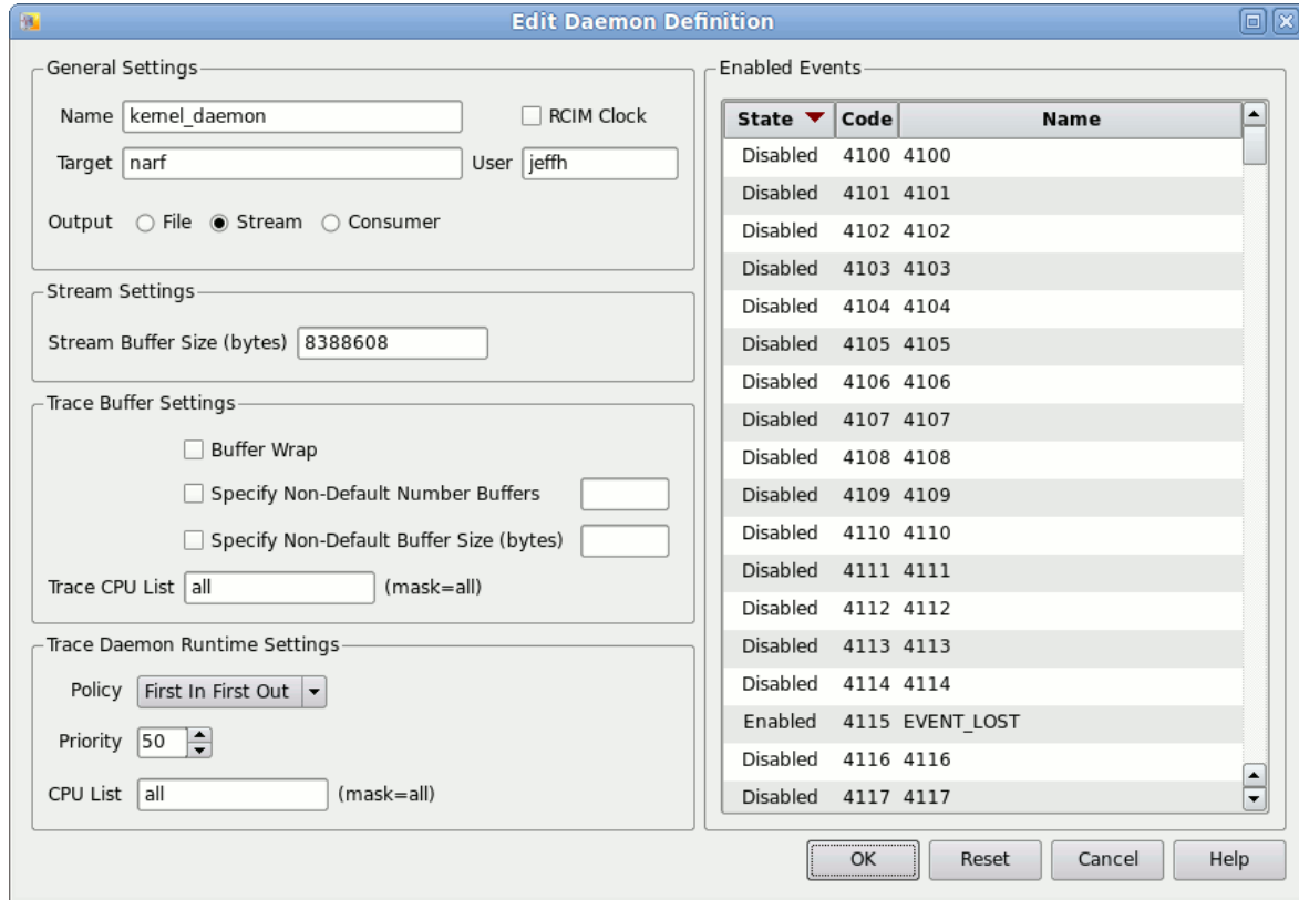
Figure 9-5. Edit Daemon Definition Dialog
