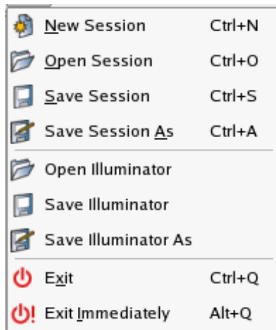
Figure 5-2. File Menu
