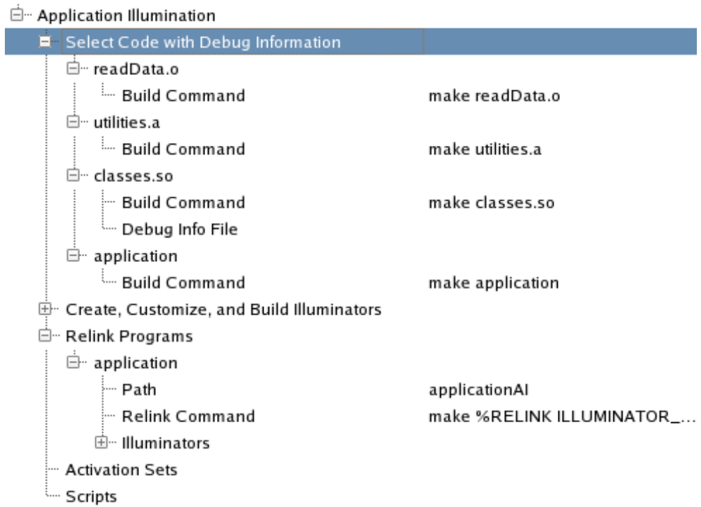
Figure 5-27. Various Objects Added to the Session Manager
