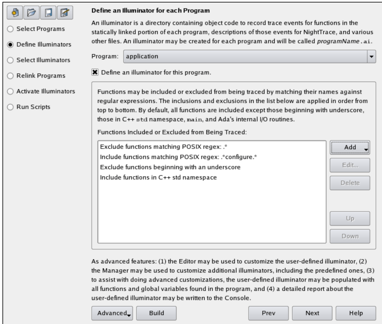
Figure 5-11. Define an Illuminator for each Program Dialog
