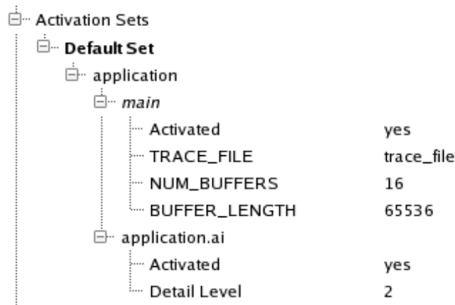
Figure 5-43. Default Options on Illuminators
