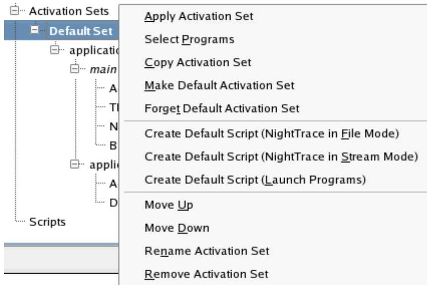
Figure 5-48. Context Menu on an Activation Set
