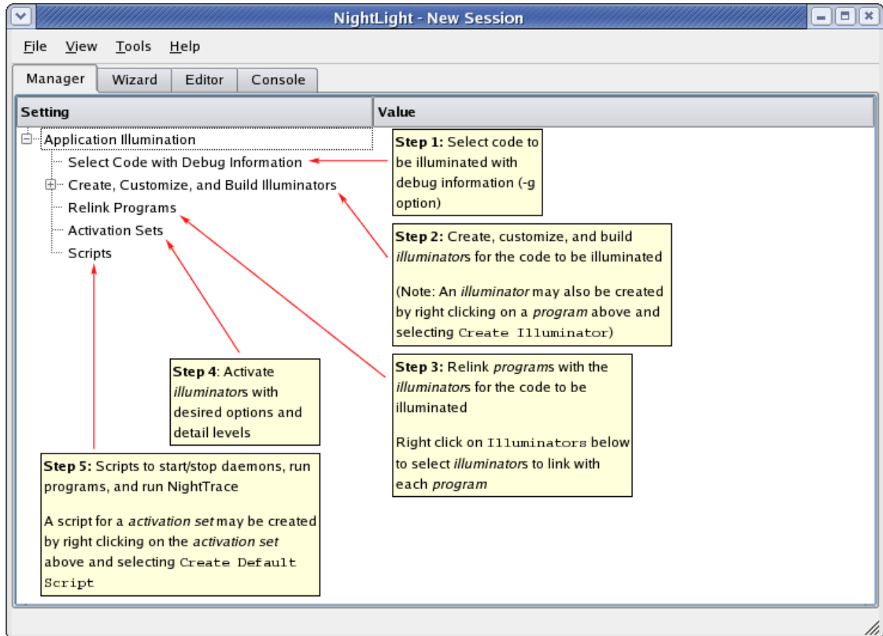
Figure 5-24. Tool Tips in the Session Manager
