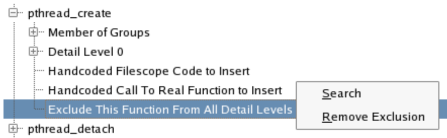
Figure 5-82. Remove Exclusion Context Menu Item
