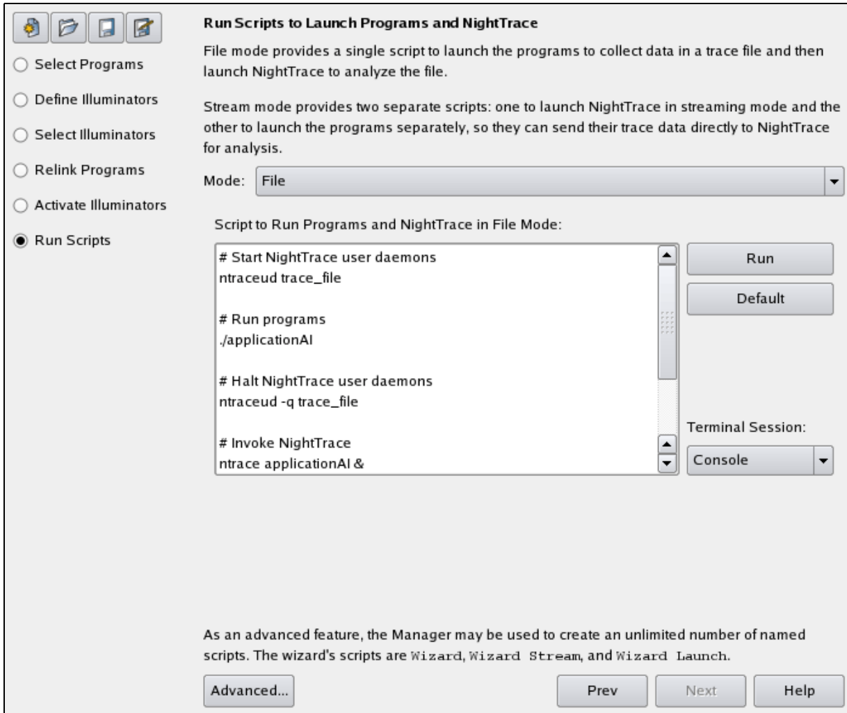
Figure 5-20. Run Scripts to Launch Programs and NightTrace Dialog in File Mode
