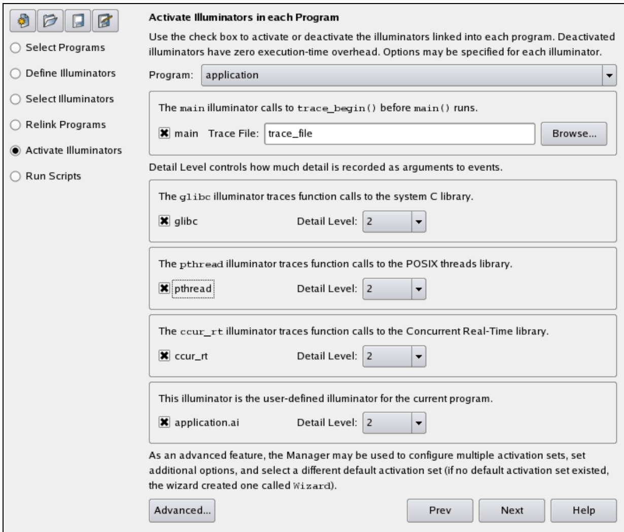
Figure 5-17. Activate Illuminators in each Program Dialog
