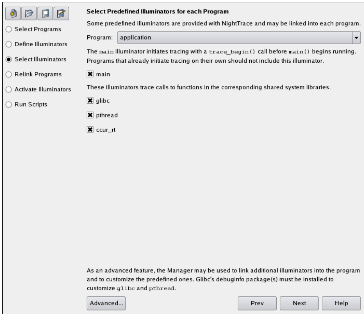
Figure 5-14. Select Predefined Illuminators for each Program Dialog
