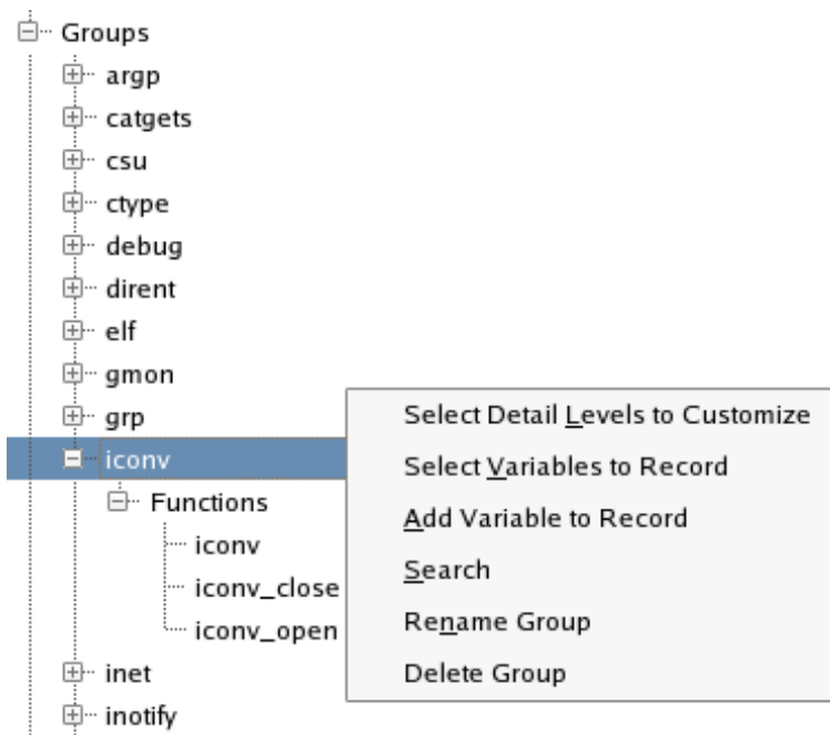
Figure 5-74. Group Name Context Menu
