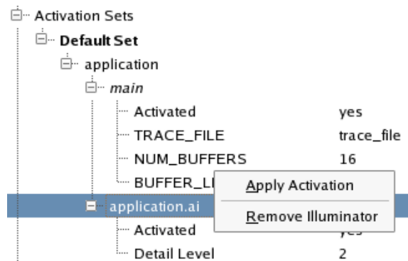
Figure 5-45. Context Menu on an Illuminator in an Activation Set
