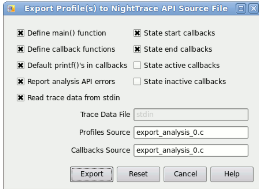
Figure 8-10. Export Profiles Dialog
