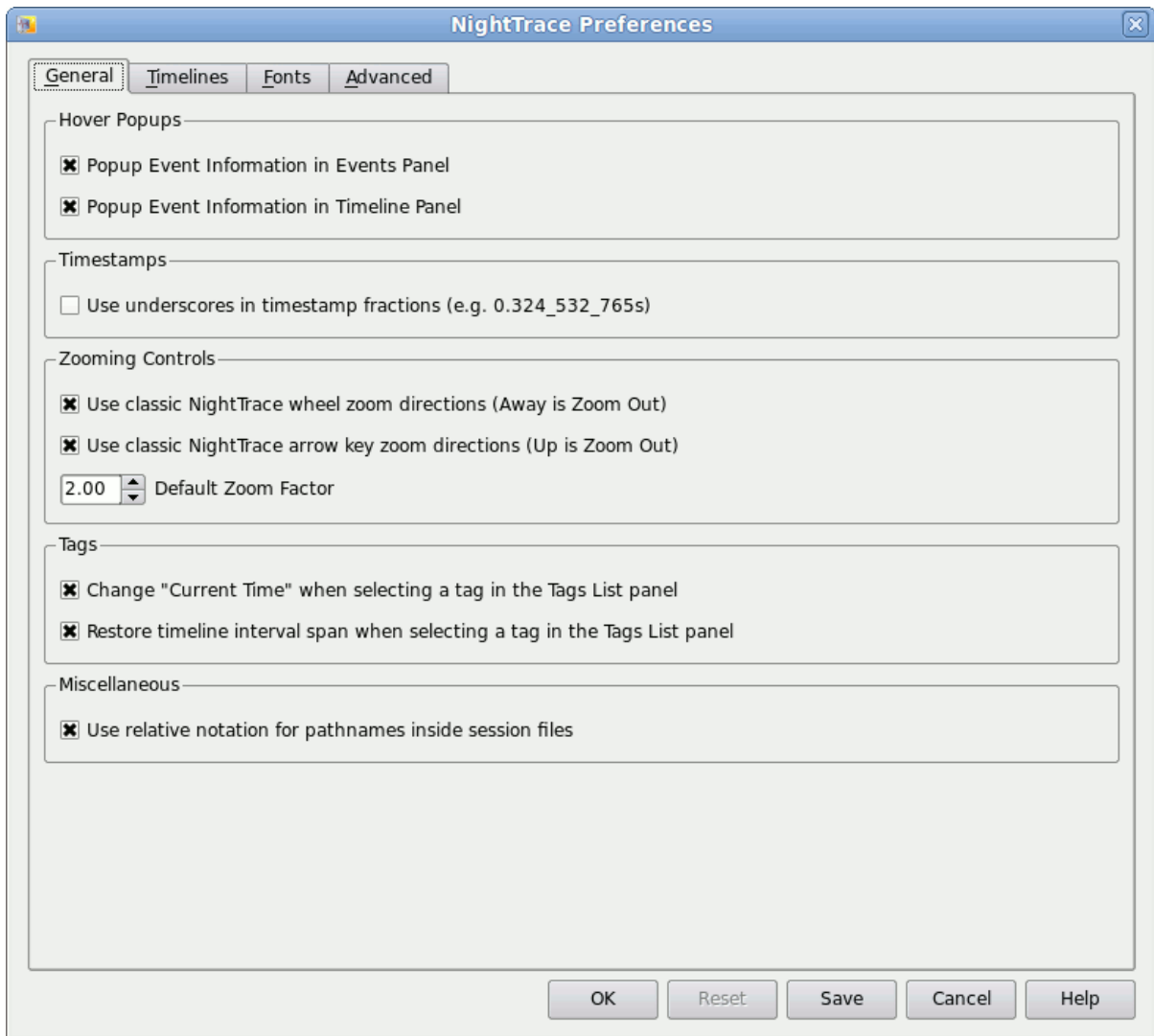
Figure 8-24. Preferences Dialog -- General Tab
