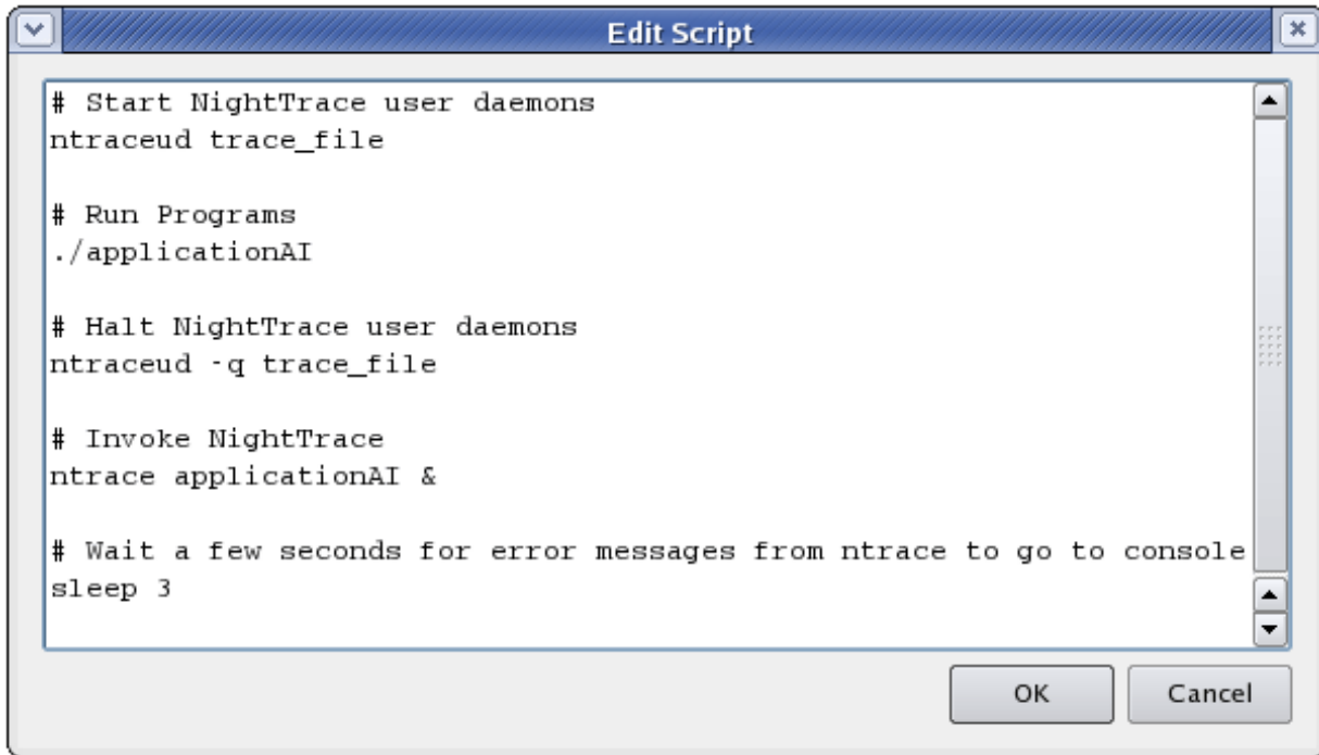
Figure 5-54. Default Script created for an Activation Set (NightTrace in File Mode)
