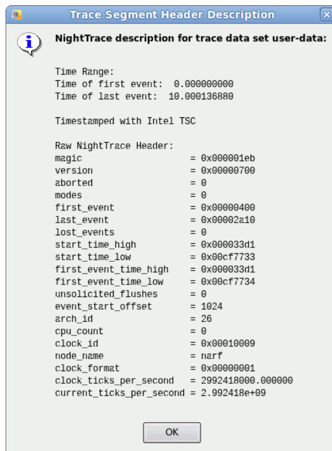
Figure 10-3. Trace Data Segment Properties Description Dialog
