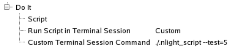
Figure 5-52. Invoking a Script on the Console While Passing an Option
