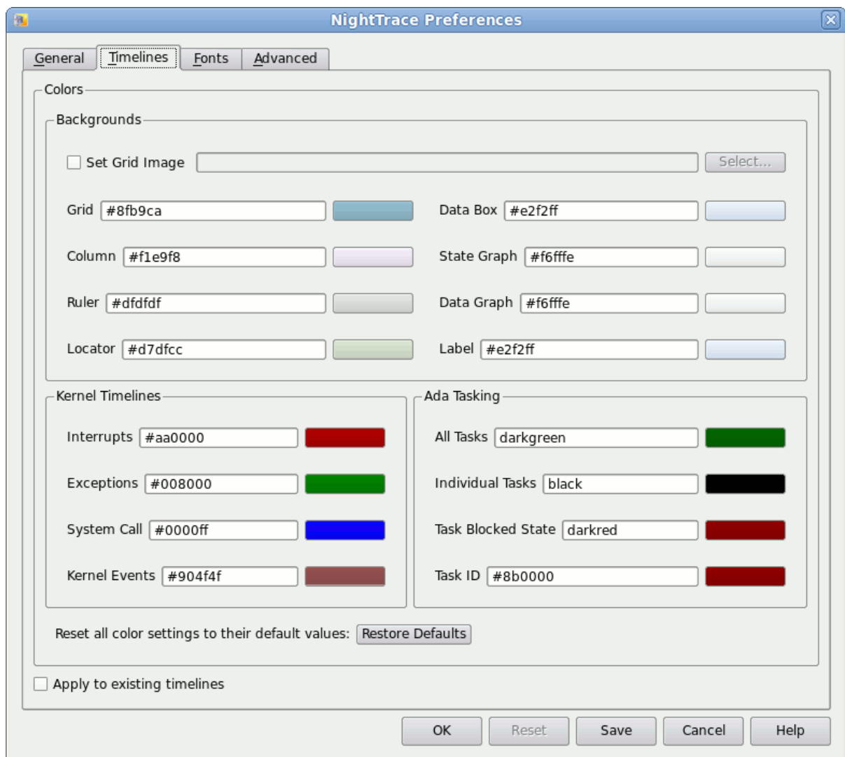
Figure 8-25. Preferences Dialog -- Timelines Tab
