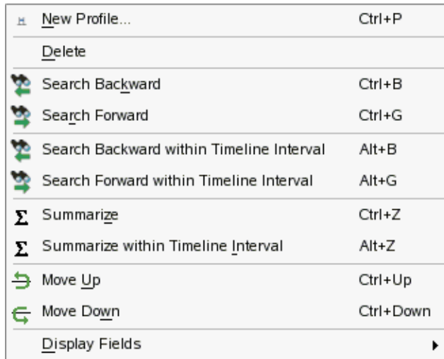
Figure 13-3. Profile Status List Panel Context Menu
