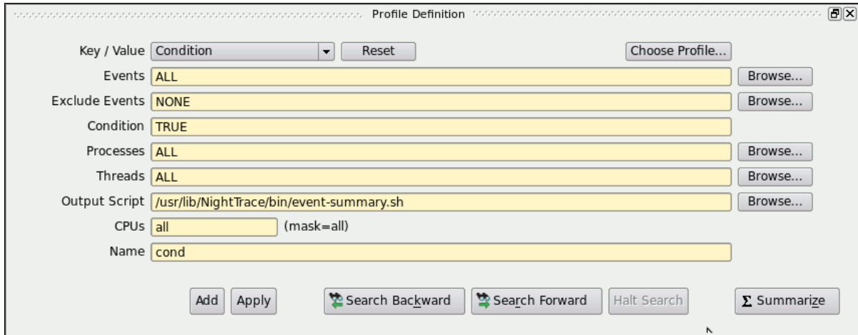
Figure 13-1. Profile Definition Panel
