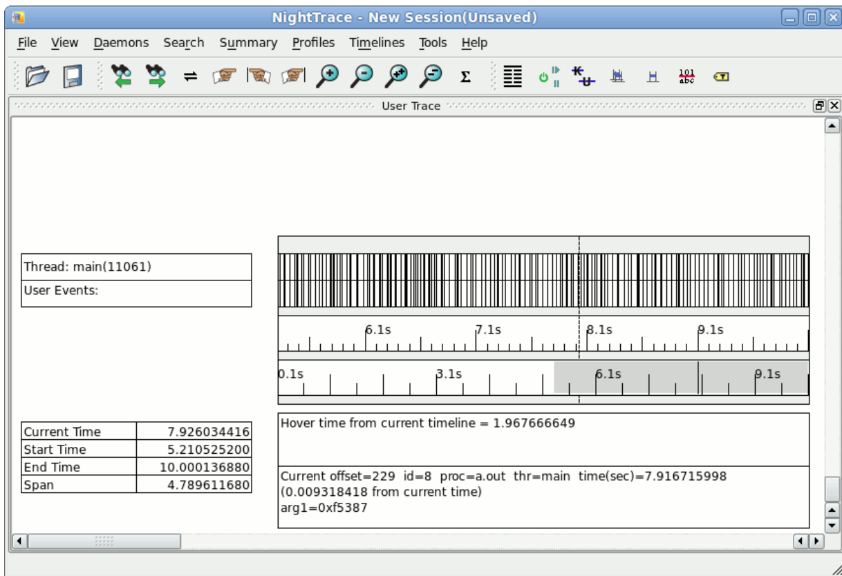
Figure 8-12. Default User Timeline
