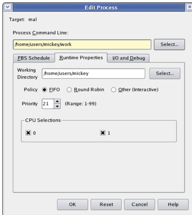
Figure 4-18. Add Process and Edit Process Dialog - Runtime Properties Page
