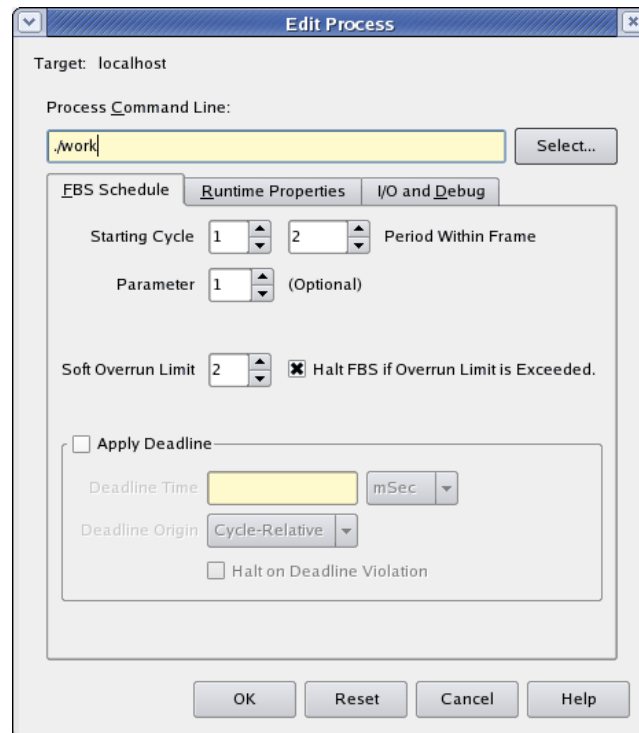
Figure 4-16. Edit Process Dialog
