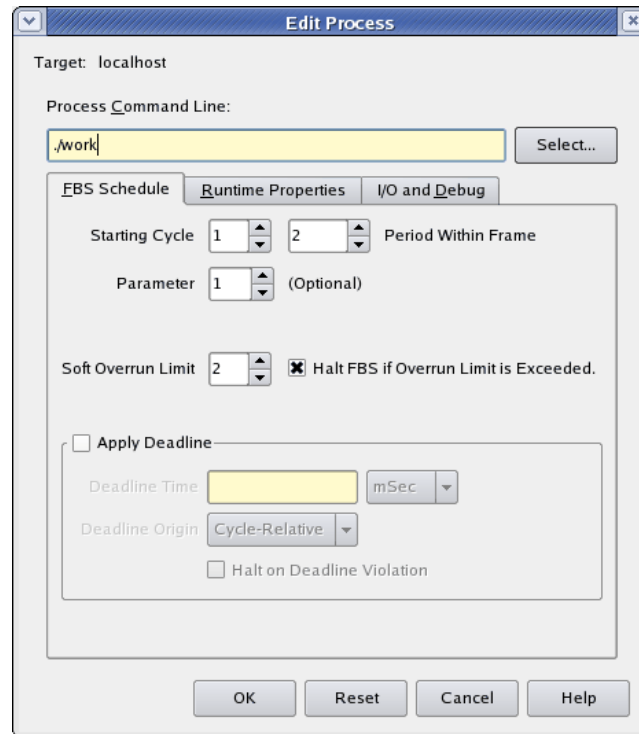
Figure 4-17. Add Process and Edit Process Dialogs - FBS Schedule Page
