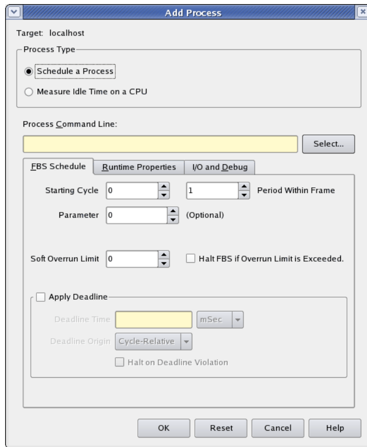
Figure 4-15. Add Process Dialog
