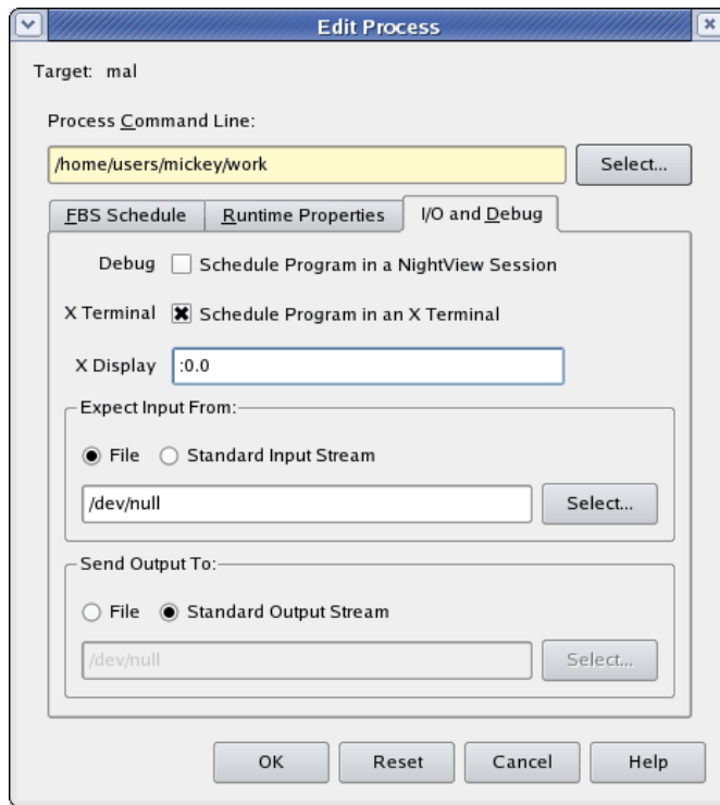
Figure 4-19. Add Process and Edit Process Dialog - I/O and Debug Page
