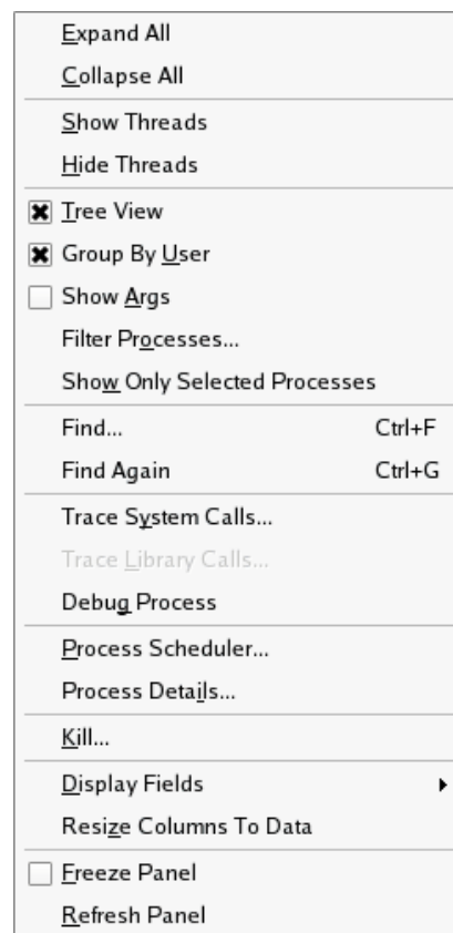
Figure 3-46. Process List Context Menu
