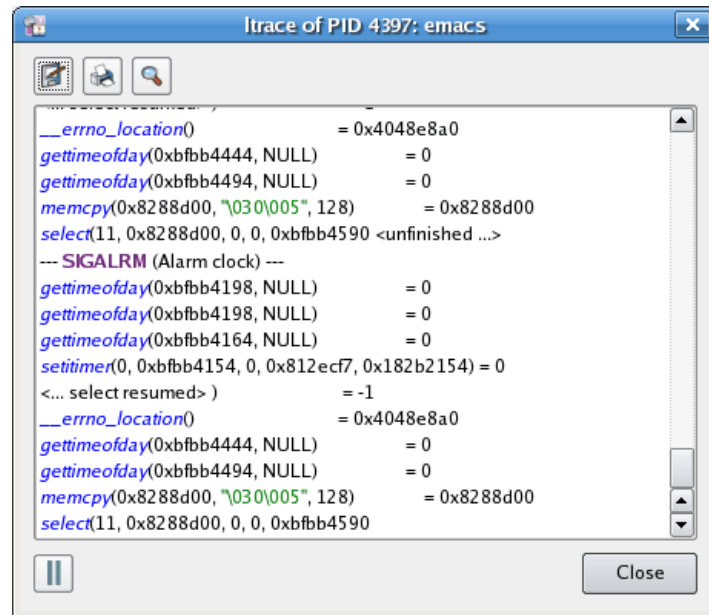
Figure 3-49. Trace Library Calls Window
