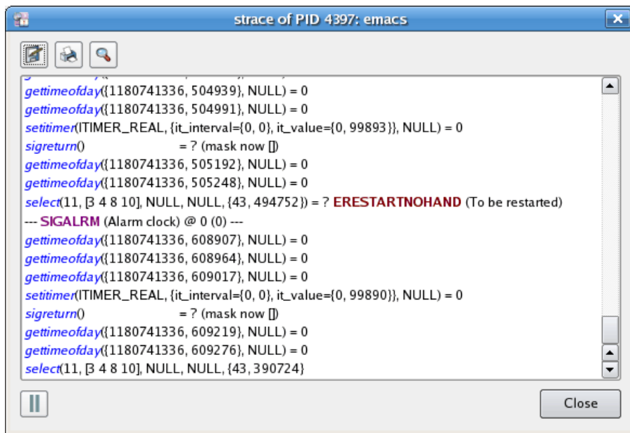
Figure 3-48. Process List Trace System Calls Window
