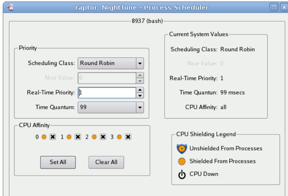
Figure 4-5. Process Scheduler Dialog
