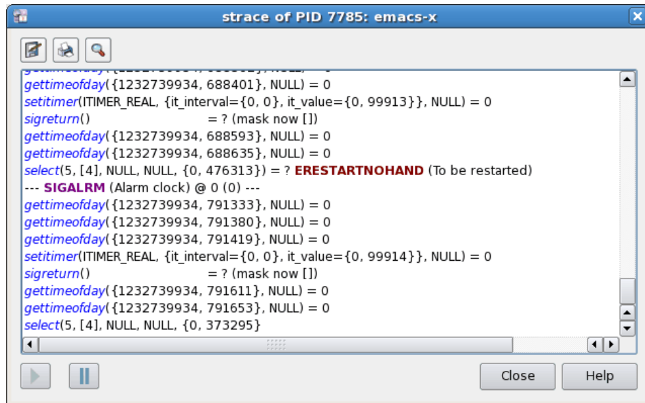
Figure 3-49. Trace Output Window
