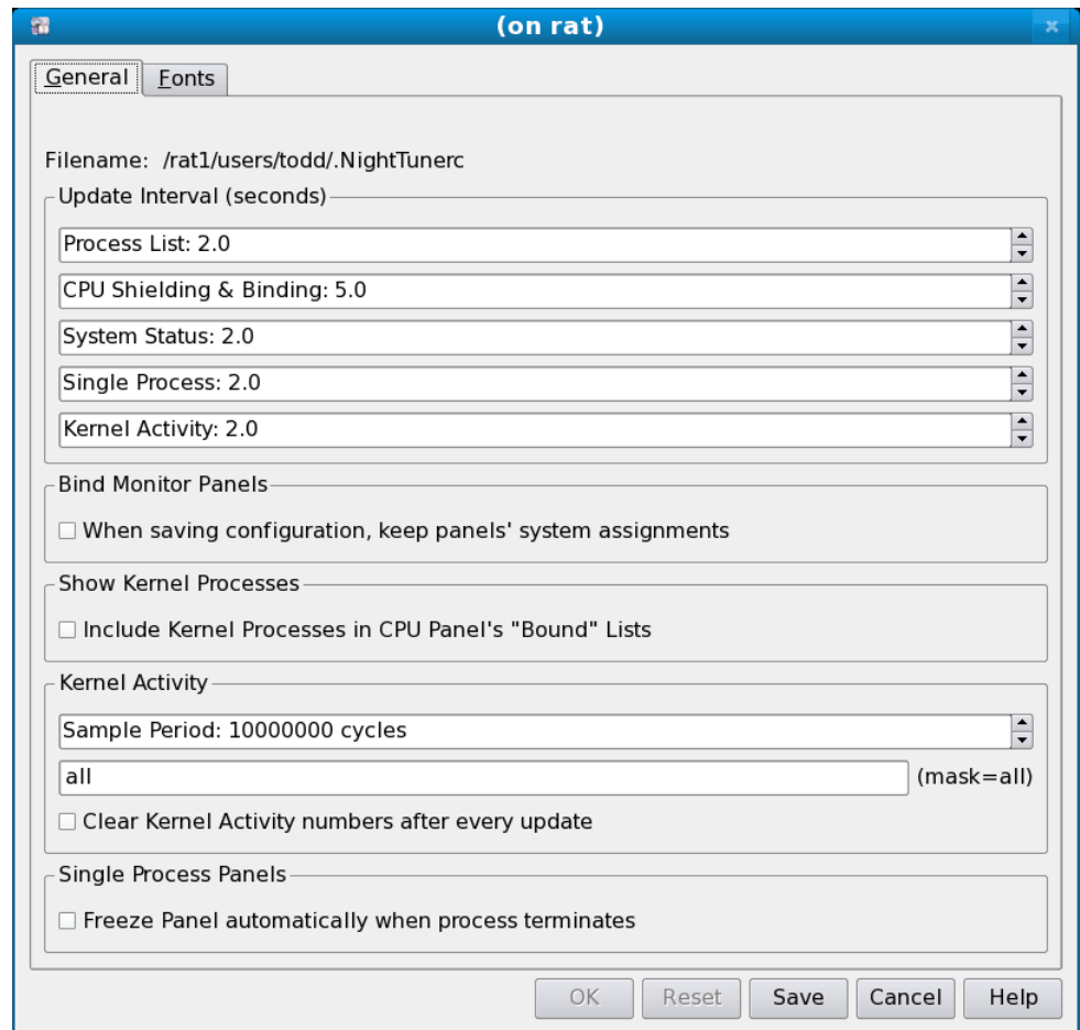
Figure 2-14. Preferences Dialog
