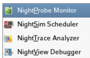
Figure 2-8. Tools Menu
