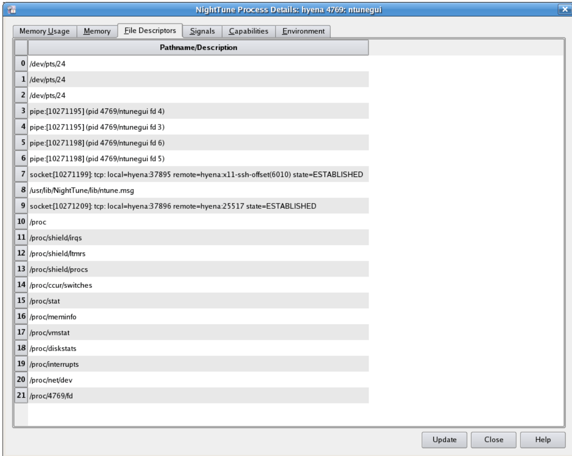
Figure 3-63. Process Details File Descriptors Tab
