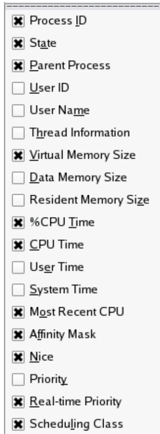
Figure 3-68. Process Fields Menu
