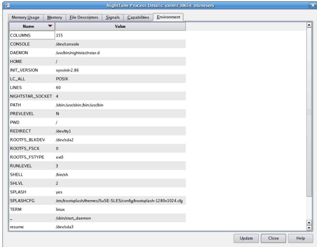
Figure 3-66. Process Details Environment Tab
