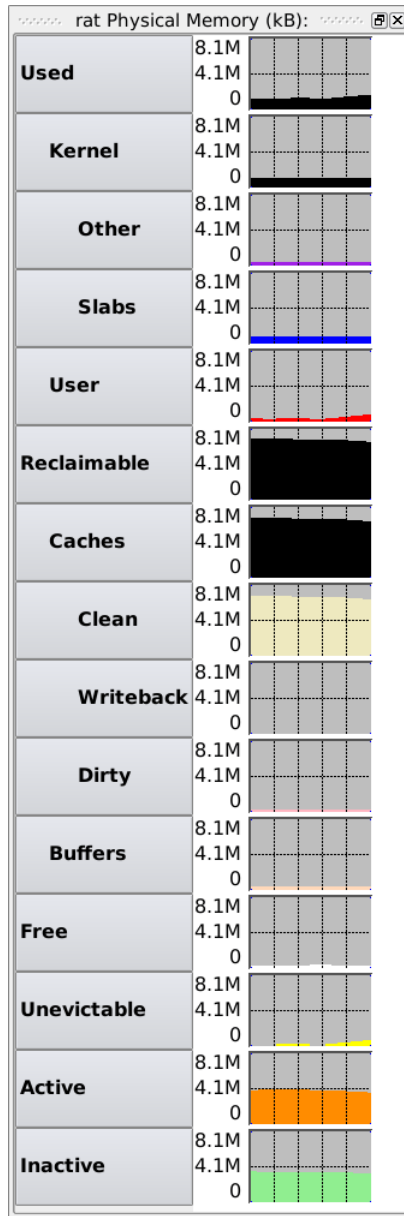
Figure 3-36. Physical Memory Line Graph Pane
