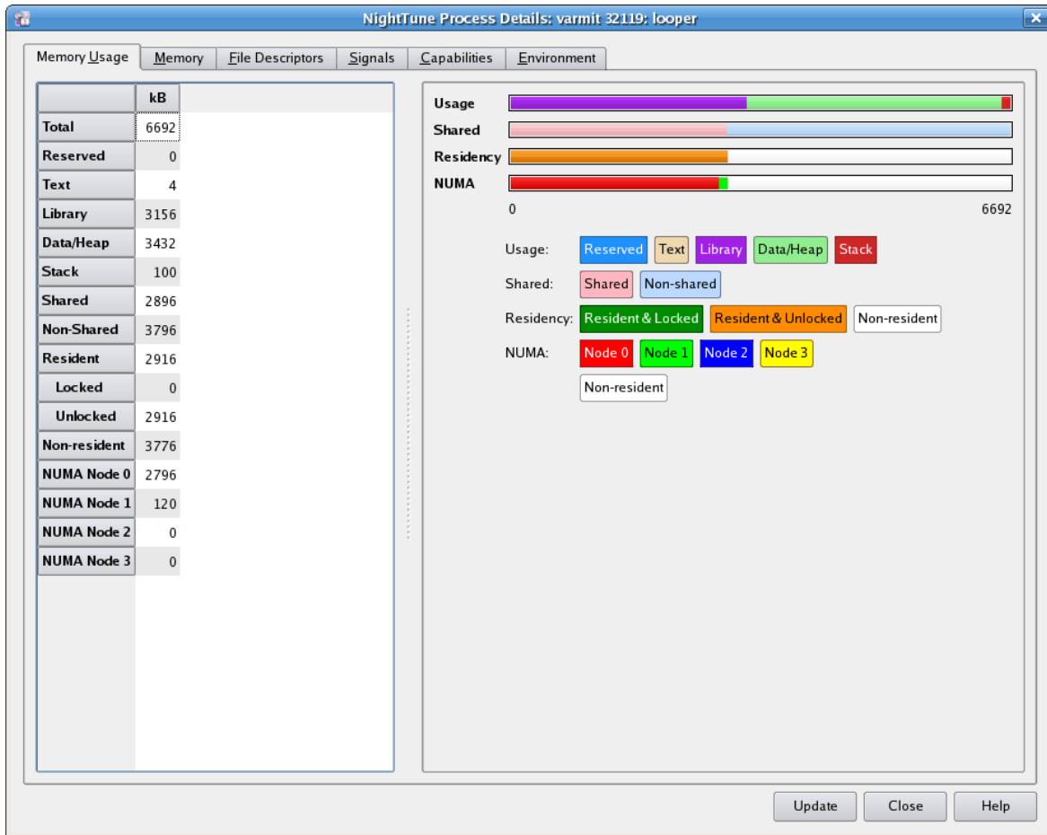
Figure 3-61. Process Details Memory Usage Tab
