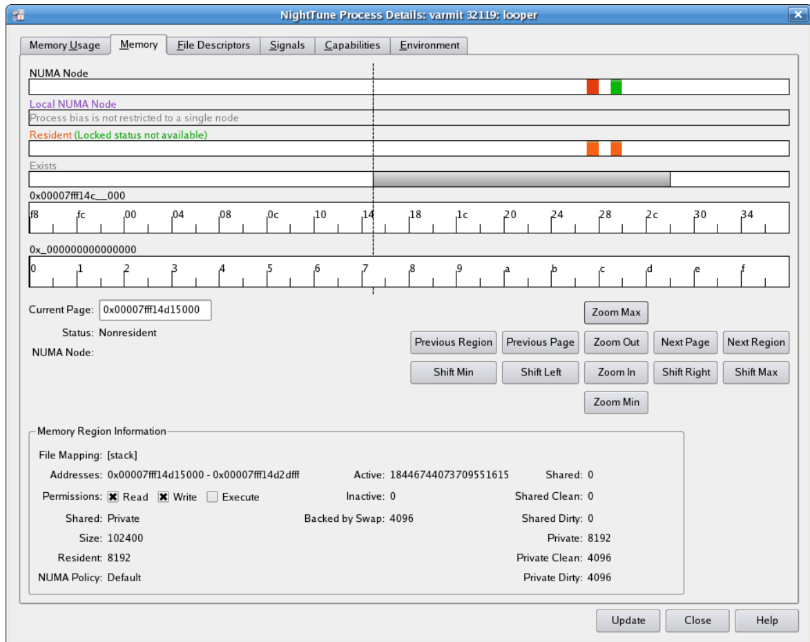
Figure 3-62. Process Details Memory Tab
