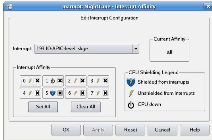
Figure 3-25. Interrupt Affinity Dialog
