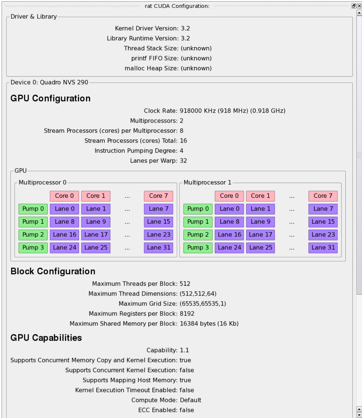
Figure 3-16. CUDA Configuration Panel
