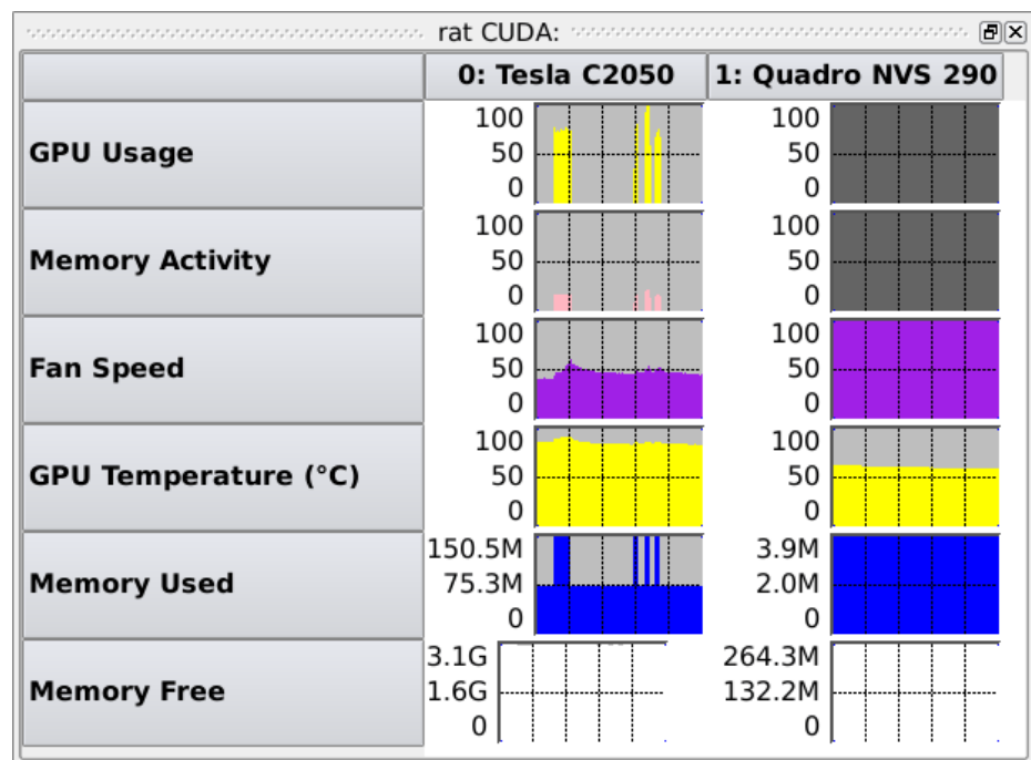
Figure 3-15. CUDA Line Graph Pane
