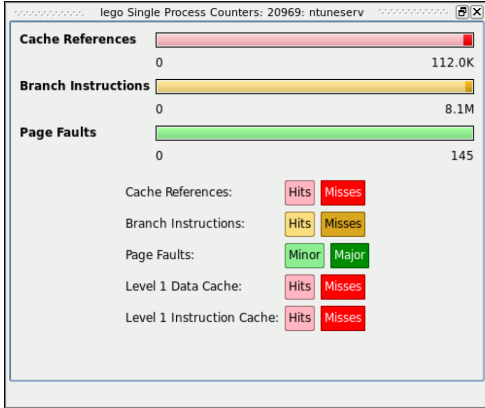
Figure 3-73. Single Process Counters Bar Graph Pane
