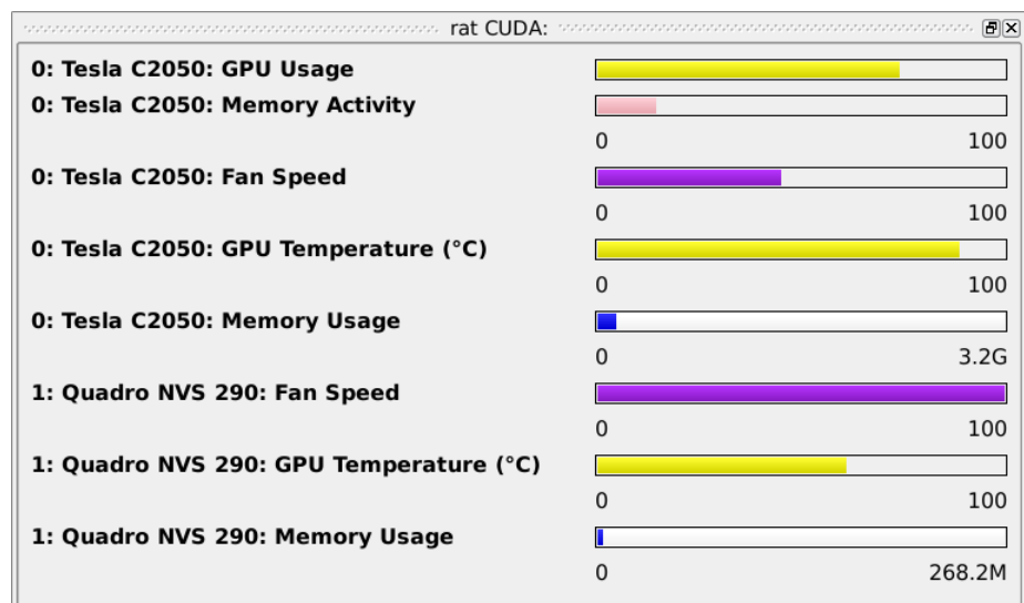
Figure 3-14. CUDA Bar Graph Pane
