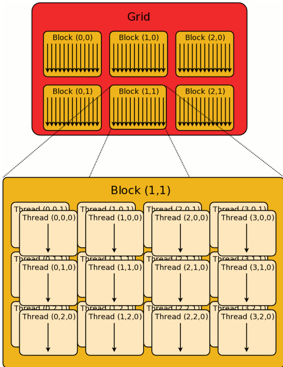
Figure 3-17. Grid, Block, and Thread Hierarchy for \langle\langle (3, 2), (4, 3, 2) \rangle\rangle
