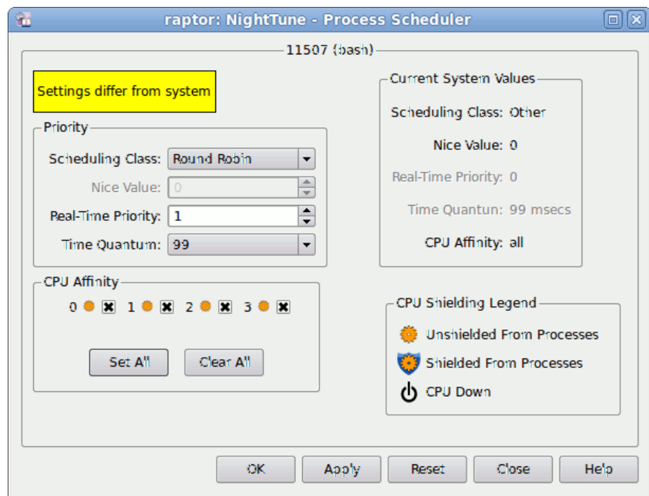
Figure 3-59. Process Scheduler Dialog
