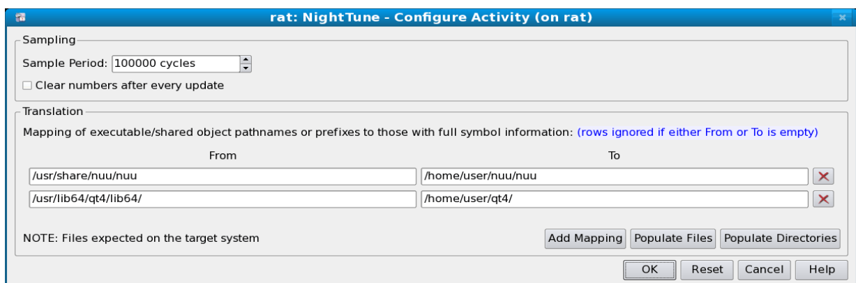
Figure 3-71. Single Process Configure Activity Dialog
