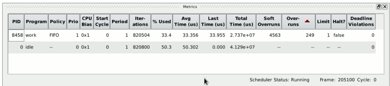
Figure 7-5. NightSim Monitor Page - Metrics Panel
