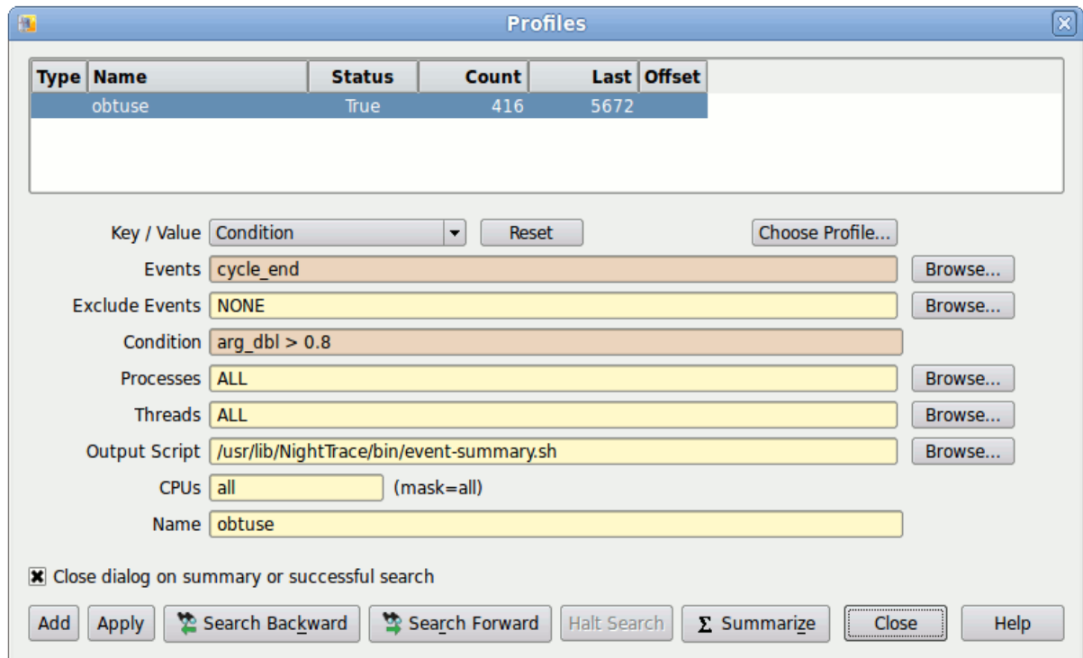
Figure 4-13. Profiles Dialog With Obtuse Profile Selected
