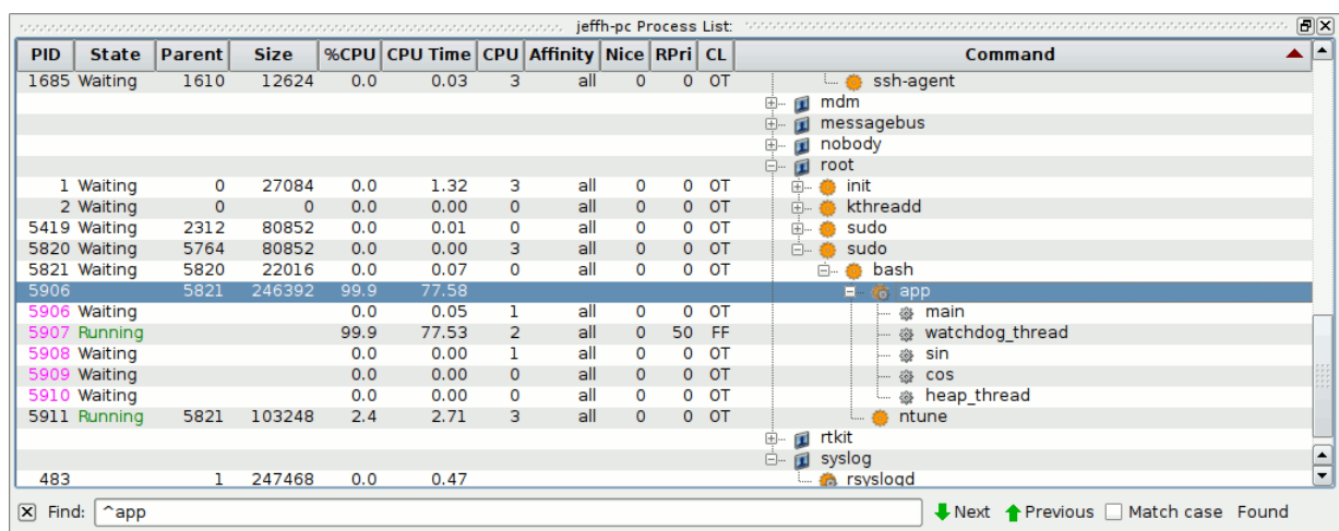
Figure 6-3. Process List with Threads
