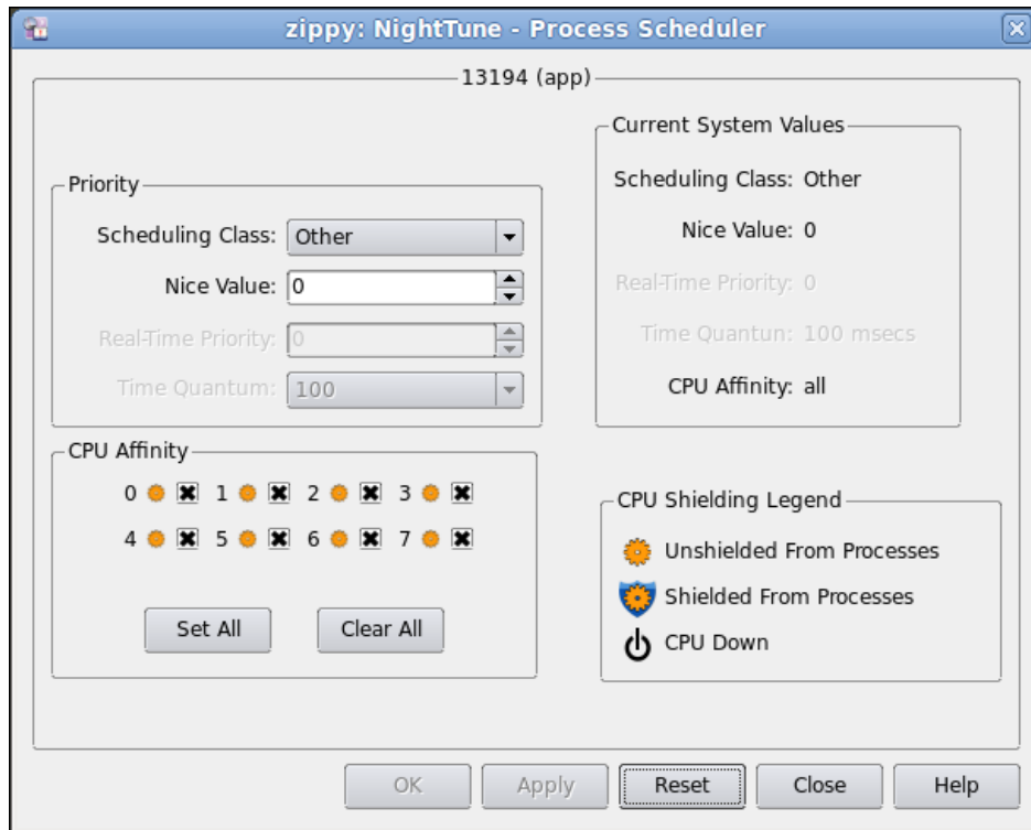
Figure 6-9. Process Scheduler Dialog
