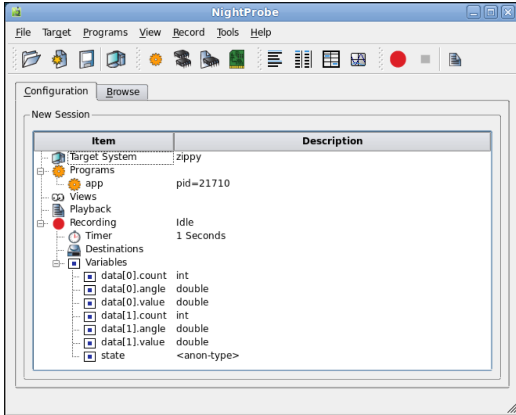
Figure 5-16. Recording area of Configuration Page
