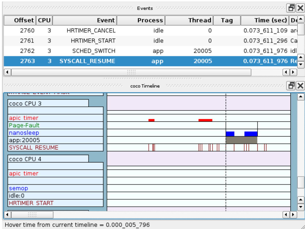
Figure 4-26. System Call Resume for Nanosleep
