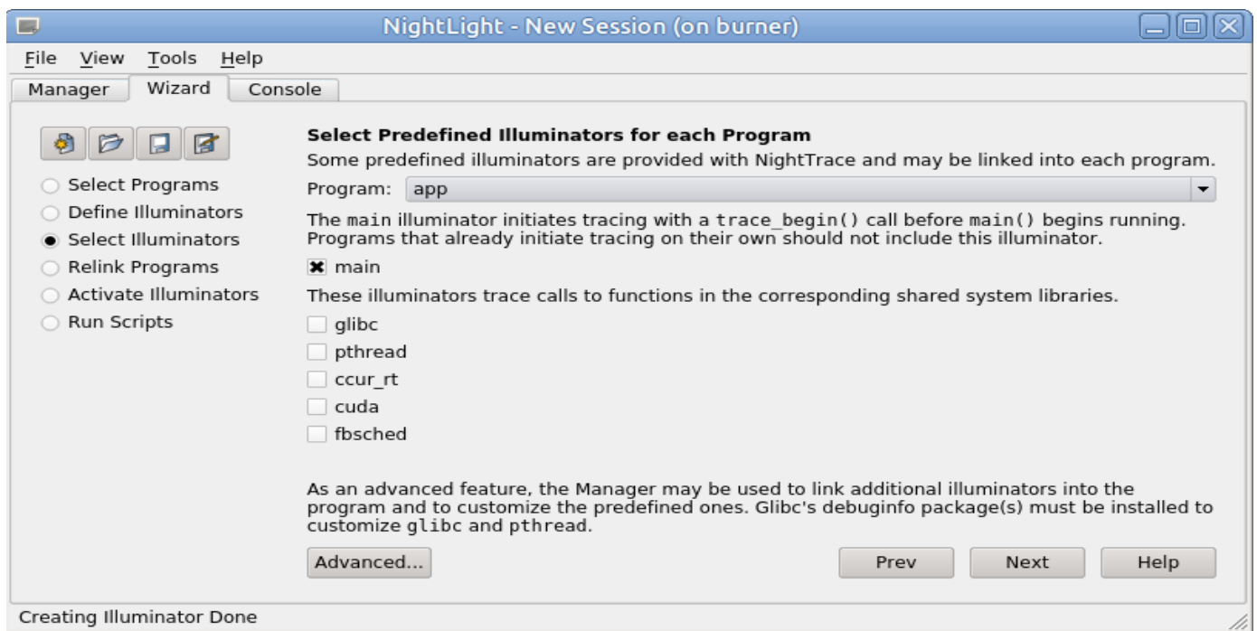
Figure 4-32. nlight Wizard - Select Illuminators Step
