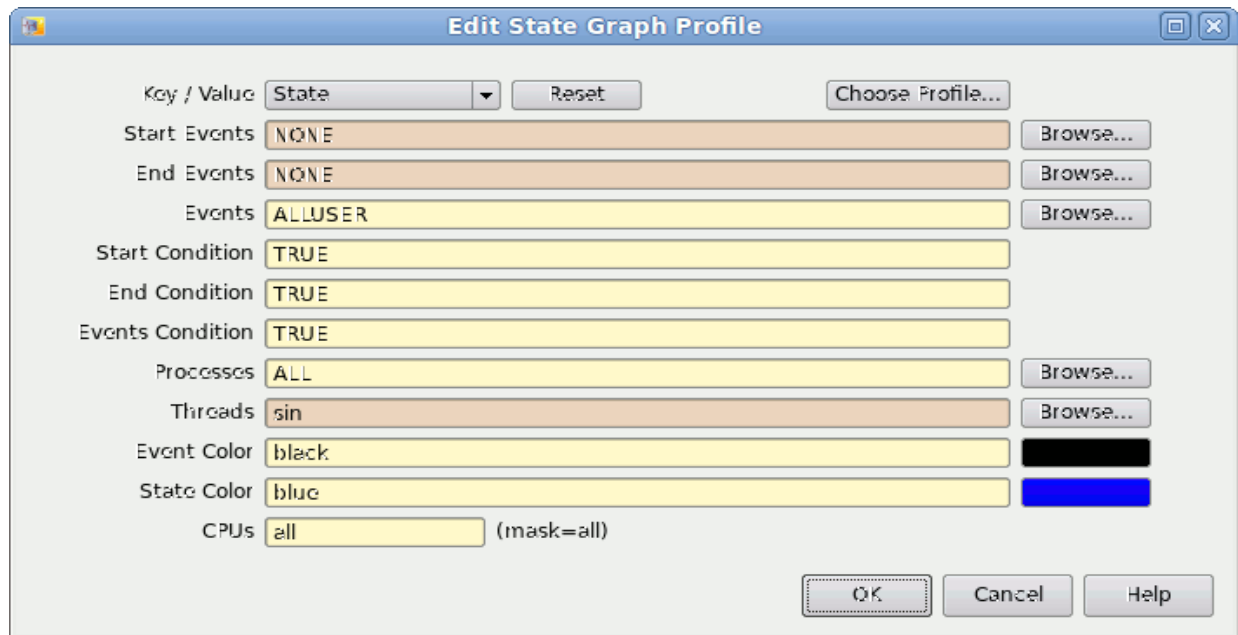
Figure 4-15. Edit State Graph Profile dialog
