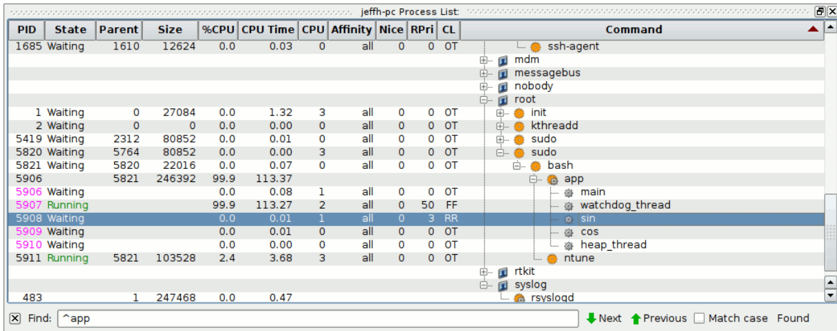
Figure 6-10. NightTune Process List with modified thread
