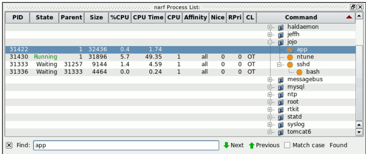
Figure 6-2. Expanded Process List
