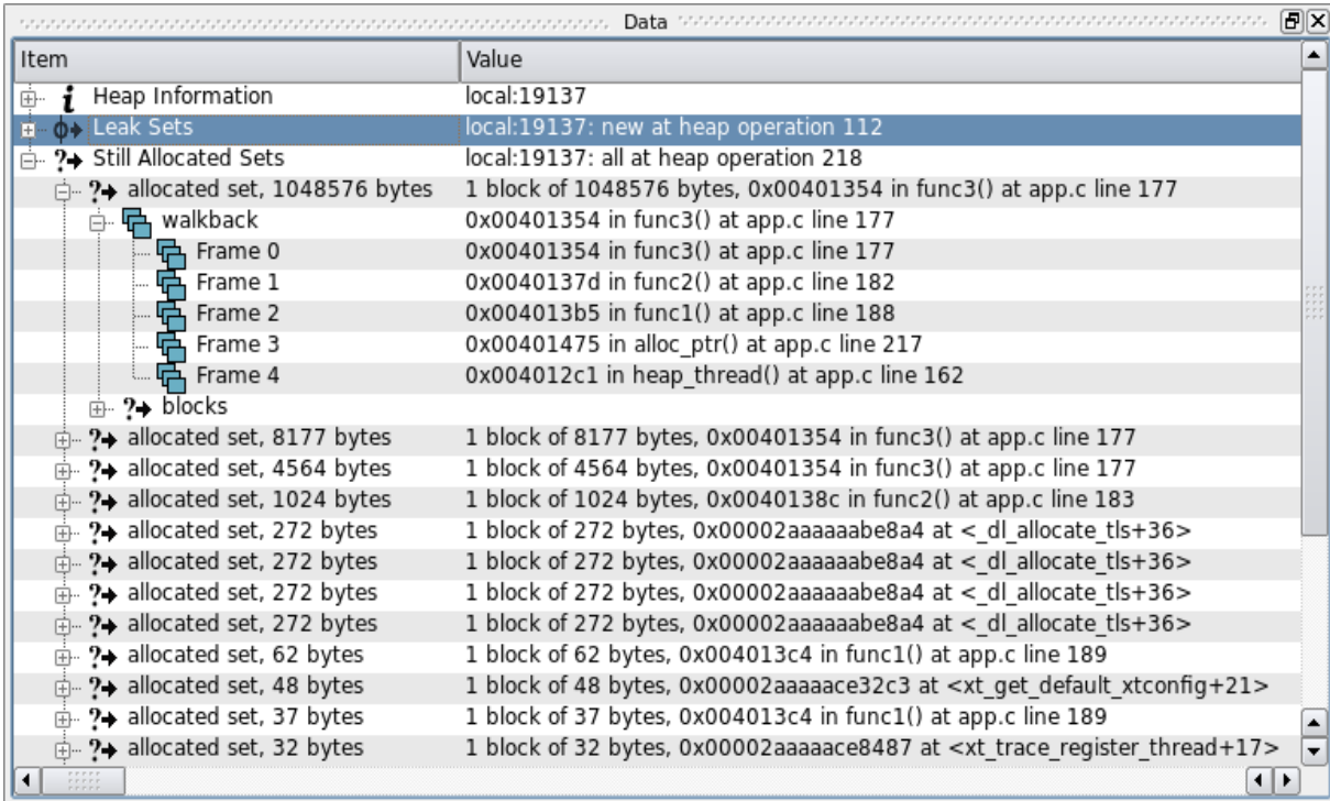
Figure 3-22. Still Allocated Blocks Display
