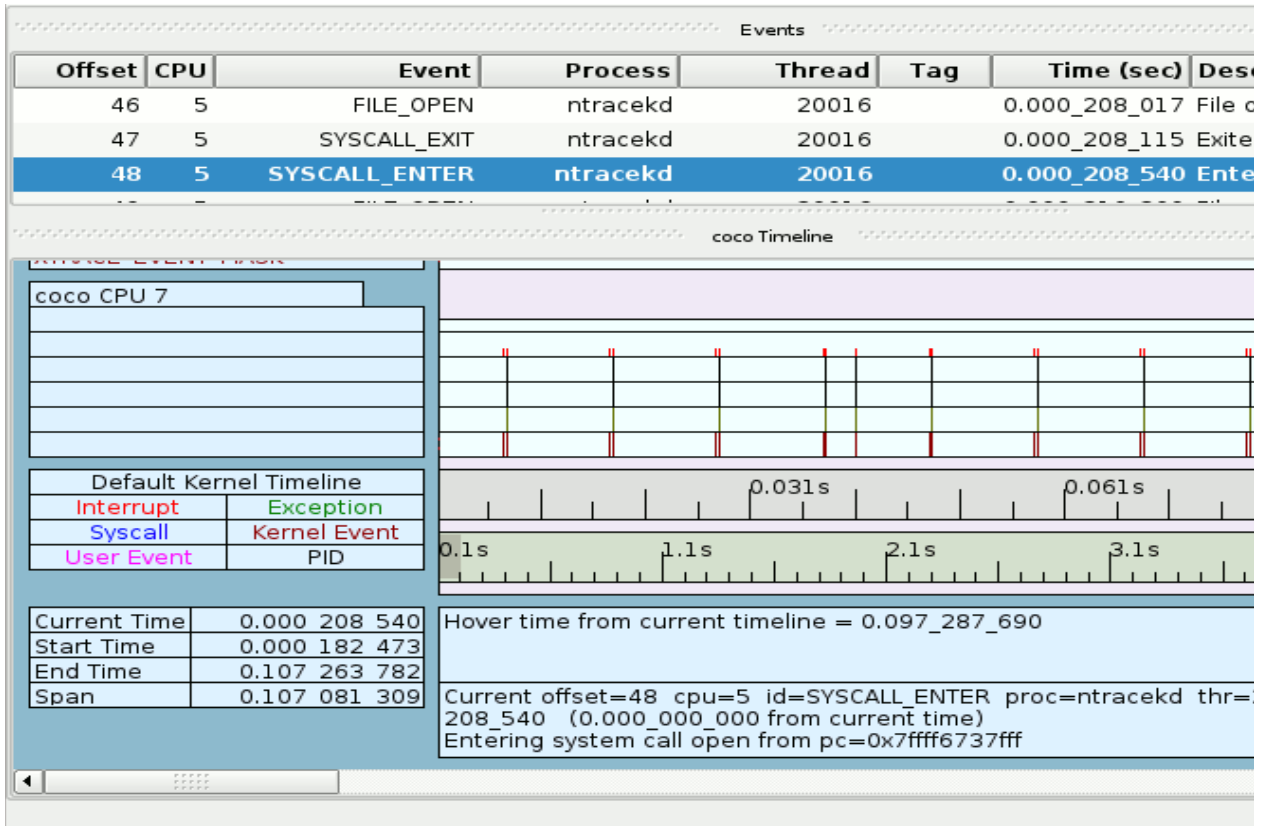
Figure 4-25. Kernel Display Page
