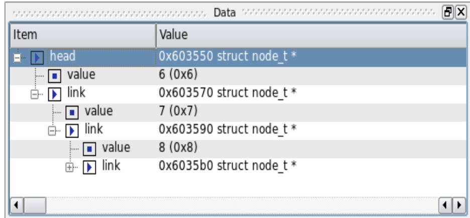
Figure 3-6. Pointer to Linked List Expanded
