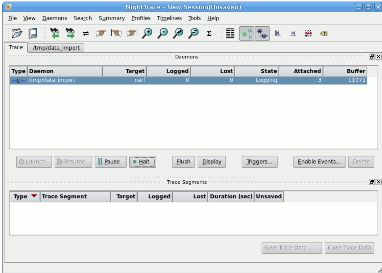
Figure 4-38. NightTrace - Daemon Collection Events
