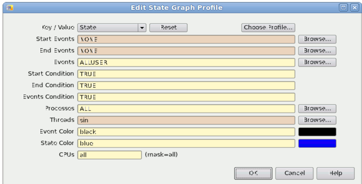
Figure 4-16. Edit State Graph Profile dialog
