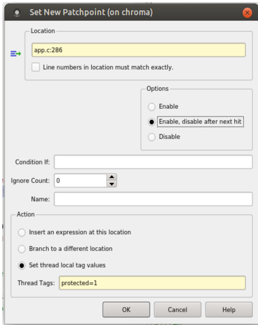
Figure 3-5. Set Patchpoint dialog with changes
