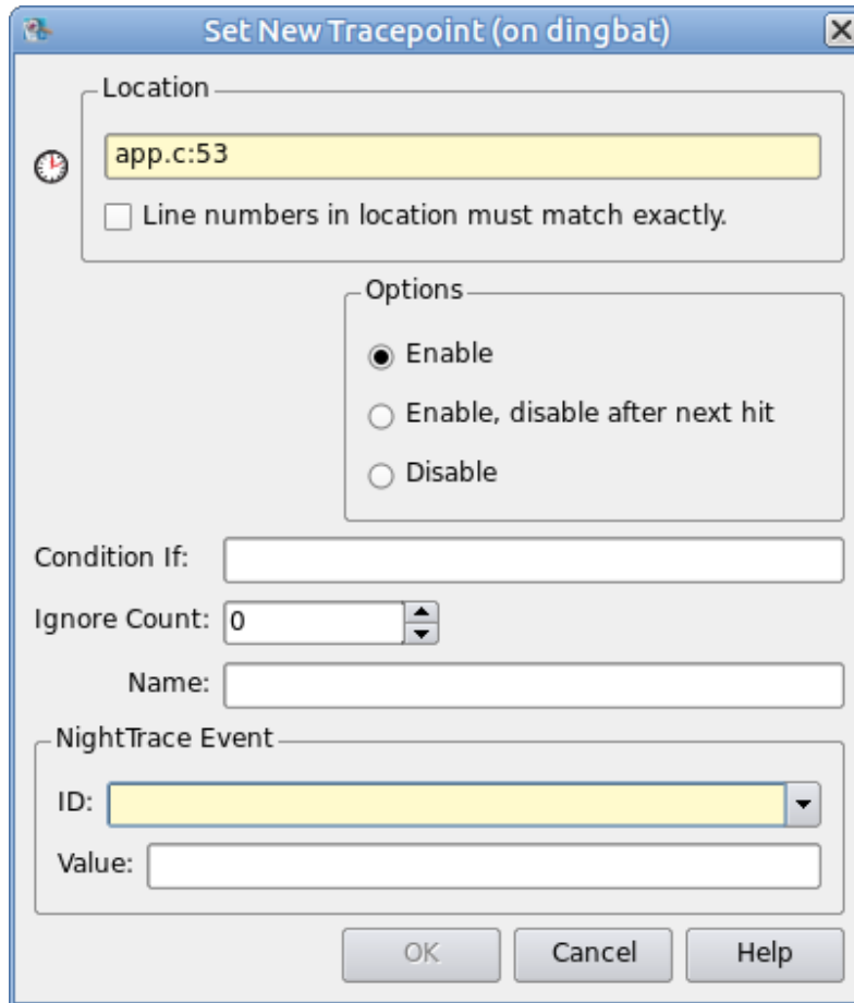
Figure 3-16. Tracepoint Dialog
