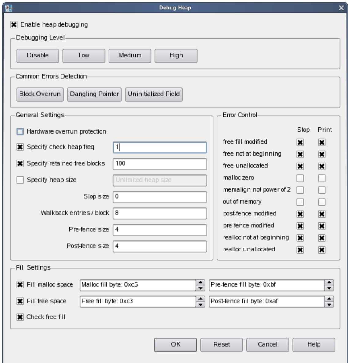
Figure 3-17. NightView Debug Heap Dialog
