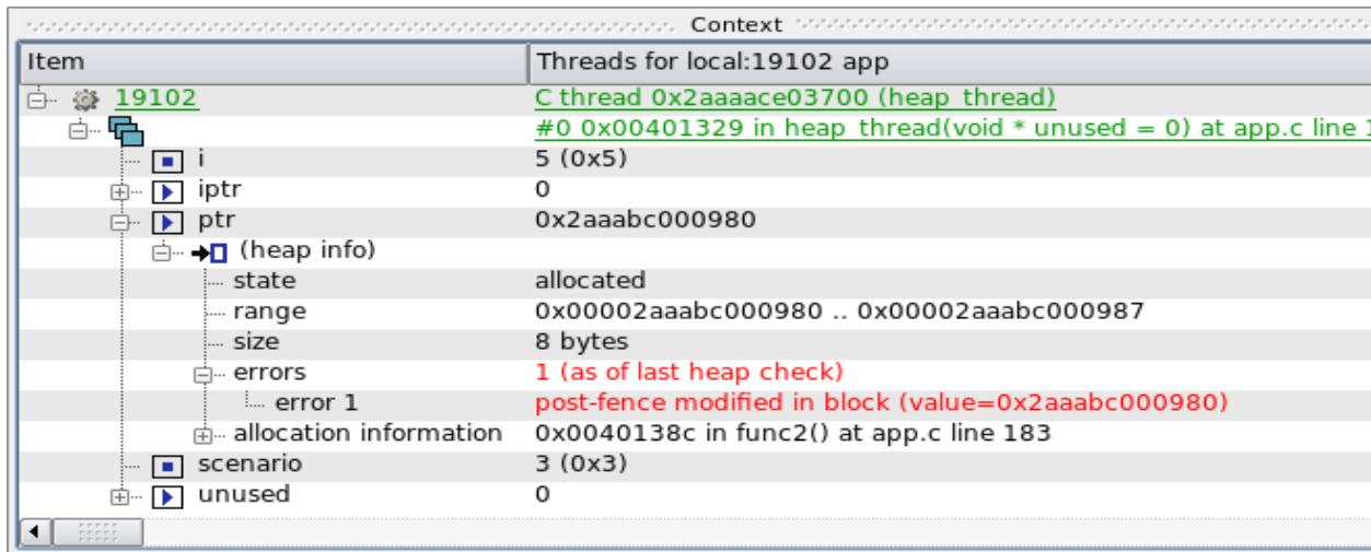
Figure 3-21. Heap Error Description
