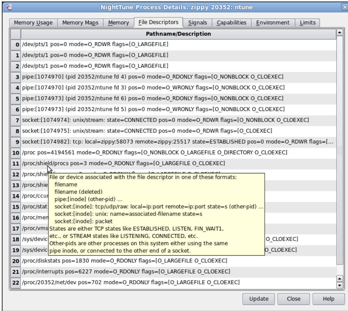
Figure 6-7. File Descriptors Page
