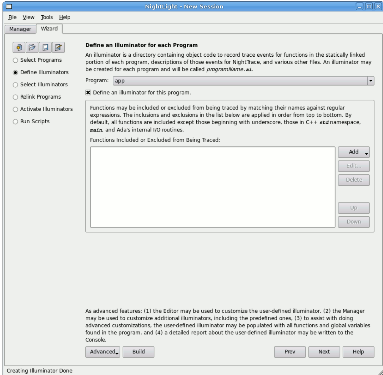
Figure 4-32. nlight Wizard - Define Illuminators Step
