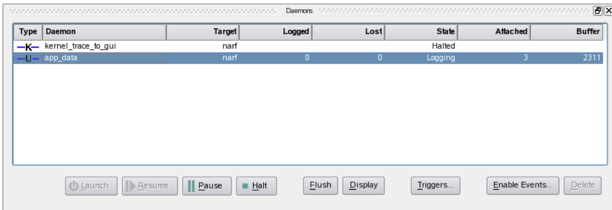
Figure 4-3. Logging Data
