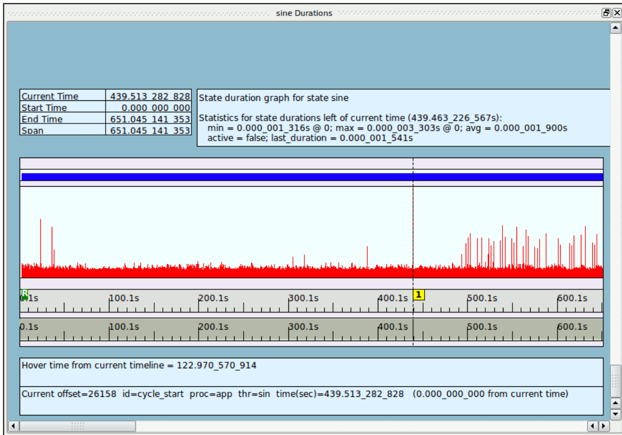
Figure 4-19. Summary Graph
