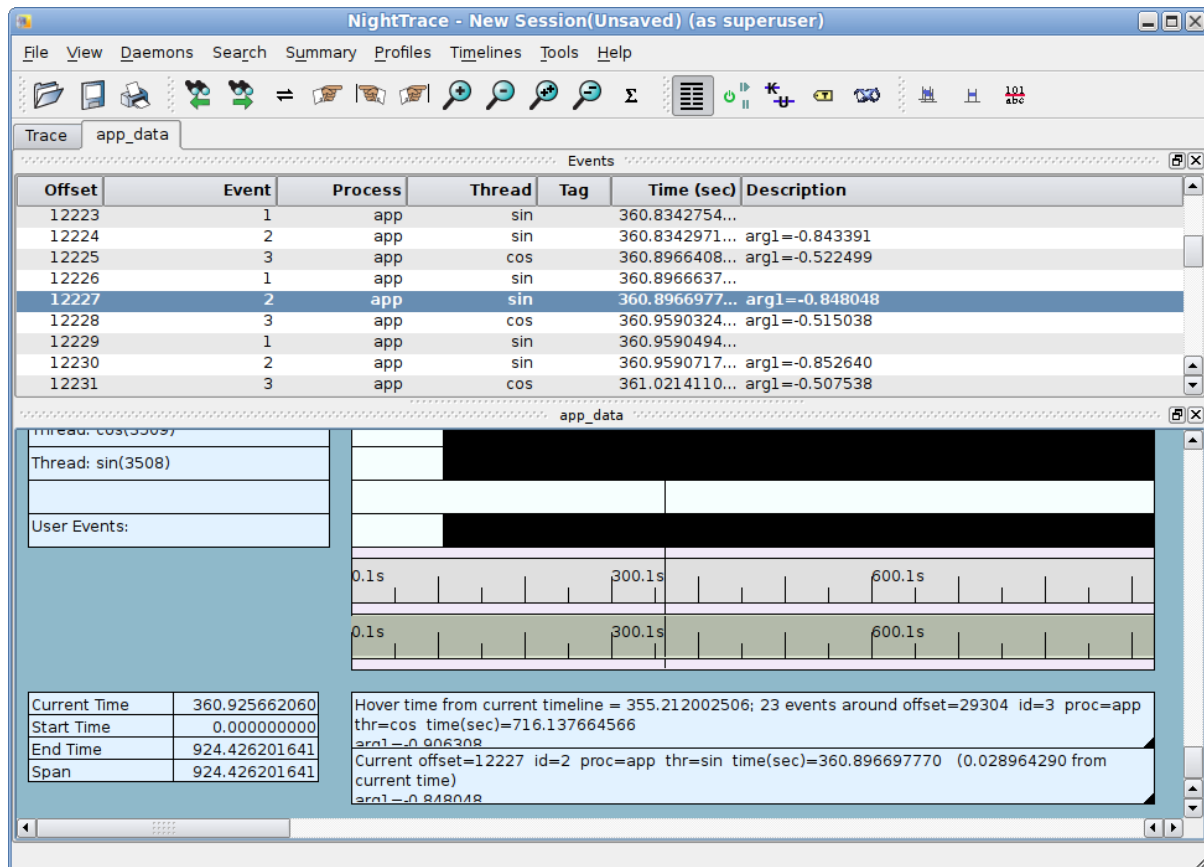
Figure 4-5. NightTrace Timeline
