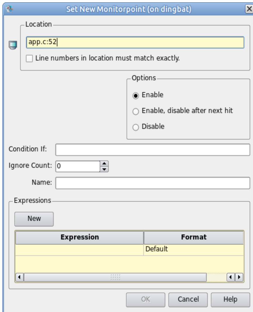
Figure 3-12. Monitorpoint Dialog
