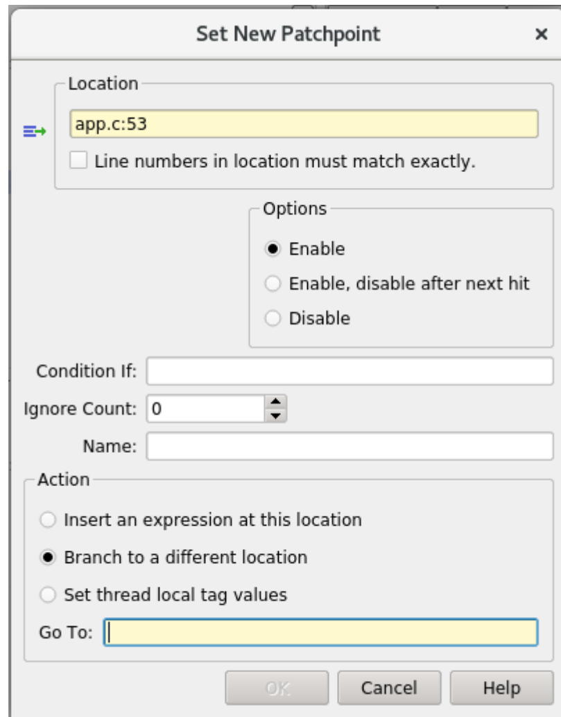
Figure 3-14. Patchpoint Dialog
