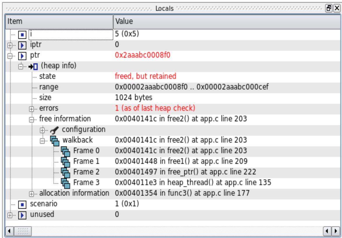
Figure 3-19. Heap Locals Info
