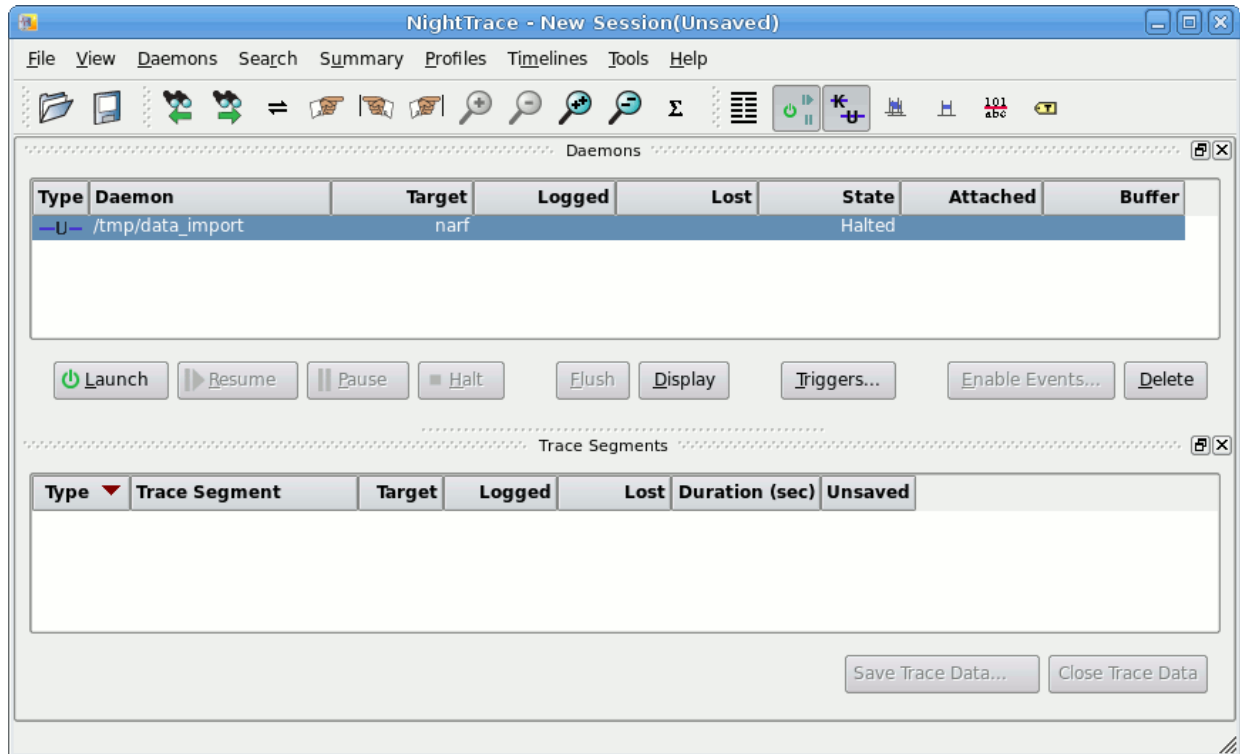
Figure 4-37. NightTrace - Daemon Ready to Launch
