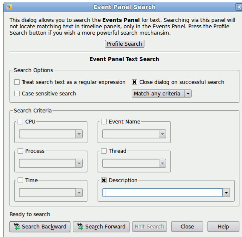
Figure 4-41. NightTrace - Event Panel Search Dialog
