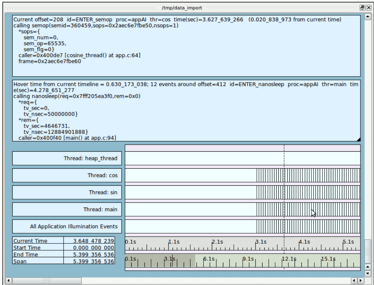
Figure 4-39. NightTrace - /tmp/data_import Timeline
