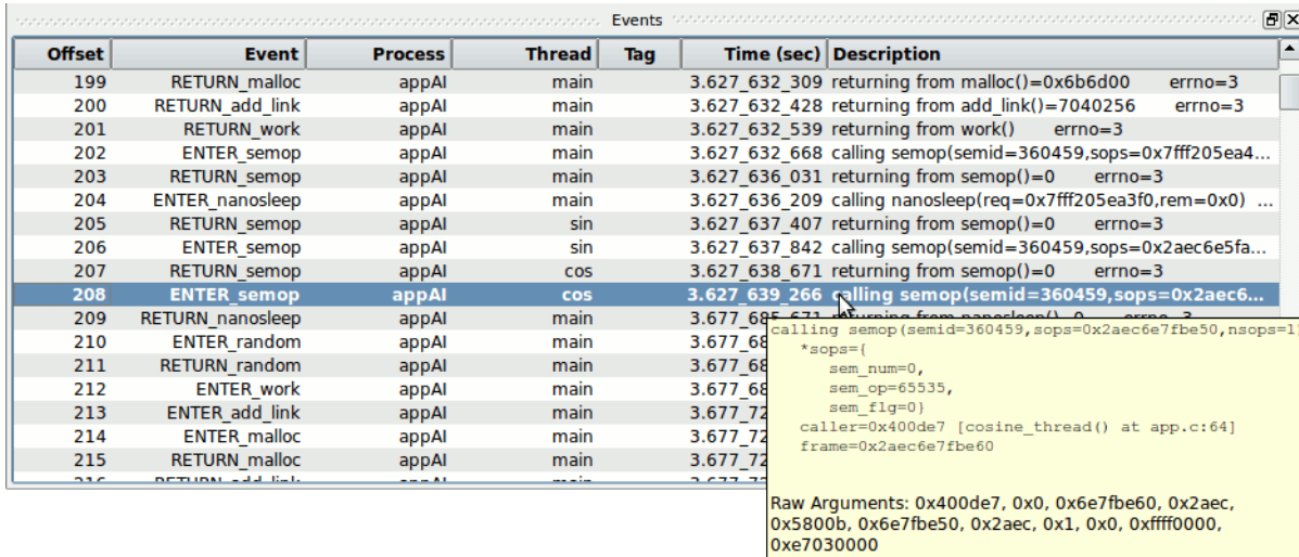
Figure 4-40. NightTrace - Events Panel w/ Tool Tip
