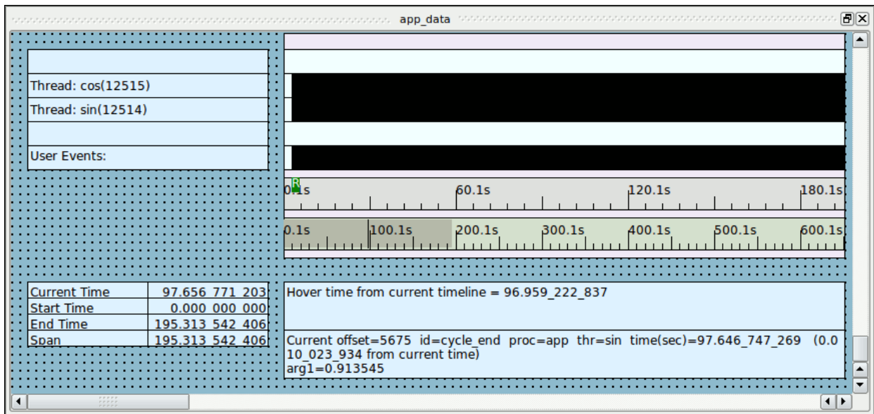
Figure 4-15. Timeline Editing
