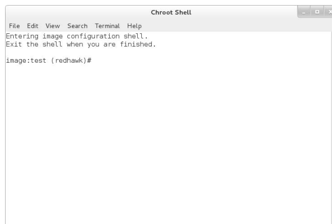
Figure 1-45 chroot Shell
