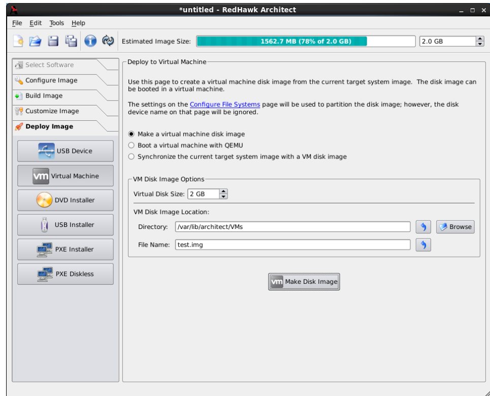
Figure 1-53 Deploy to Virtual Machine Page
