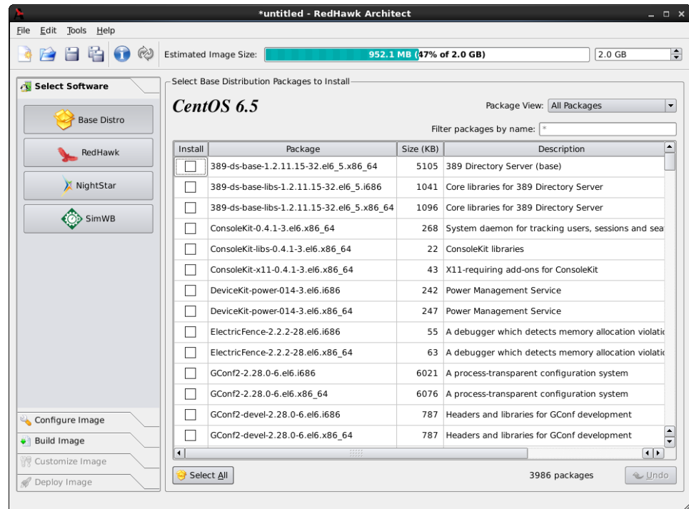
Figure 1-6 Selecting Base Distro Packages, All Packages View
