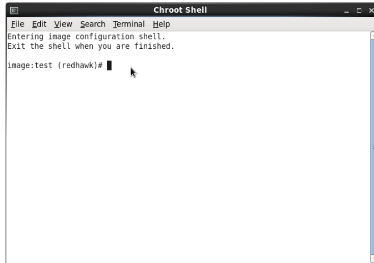
Figure 1-44 chroot Shell
