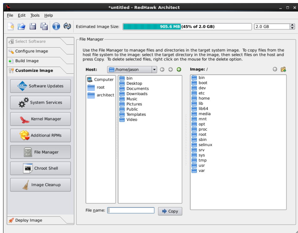
Figure 1-42 File Manager Page
