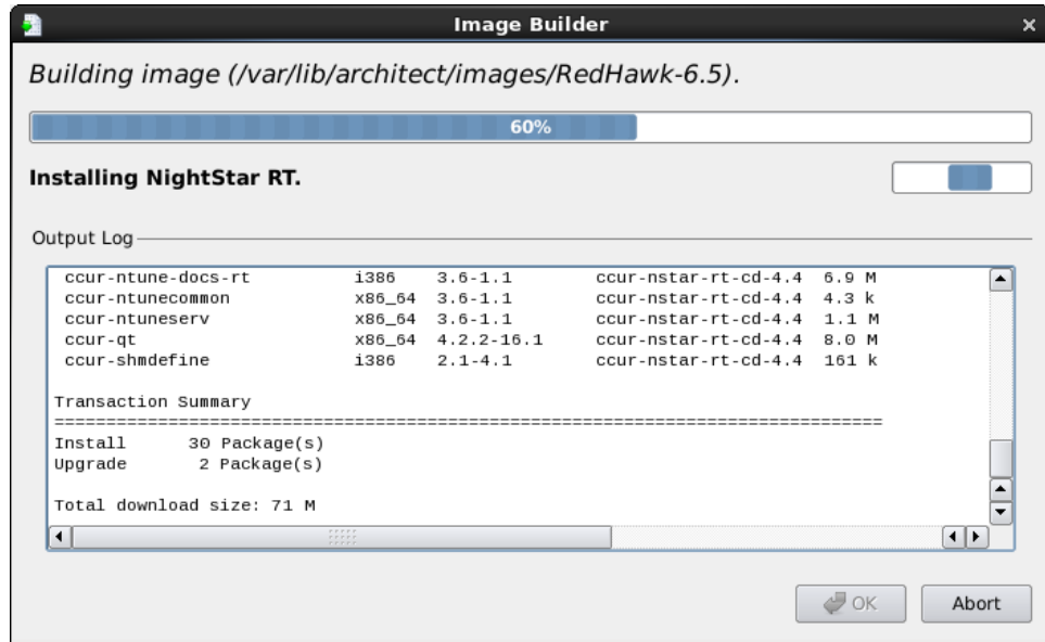
Figure 1-28 Status of NightStar Installation
