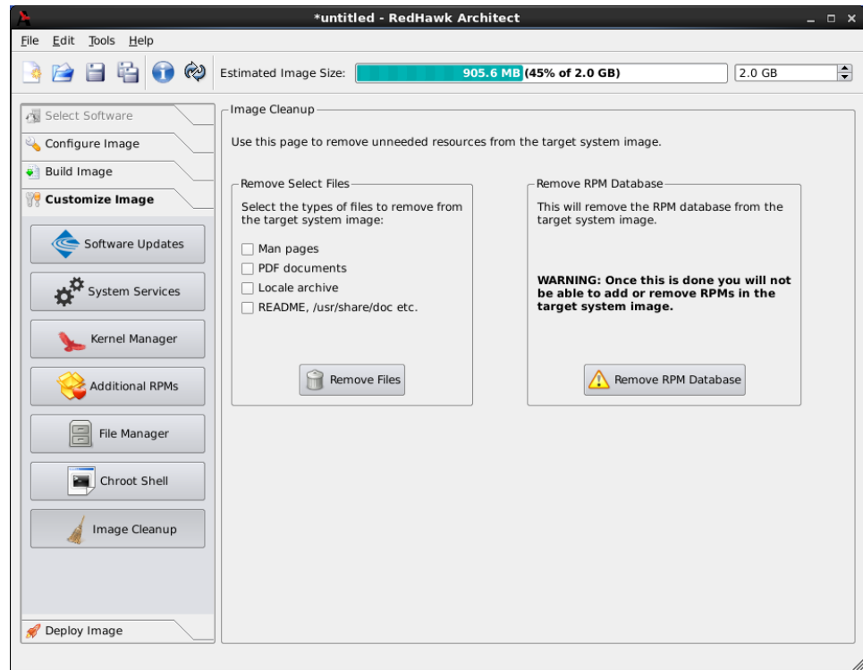
Figure 1-45 Image Cleanup Page
