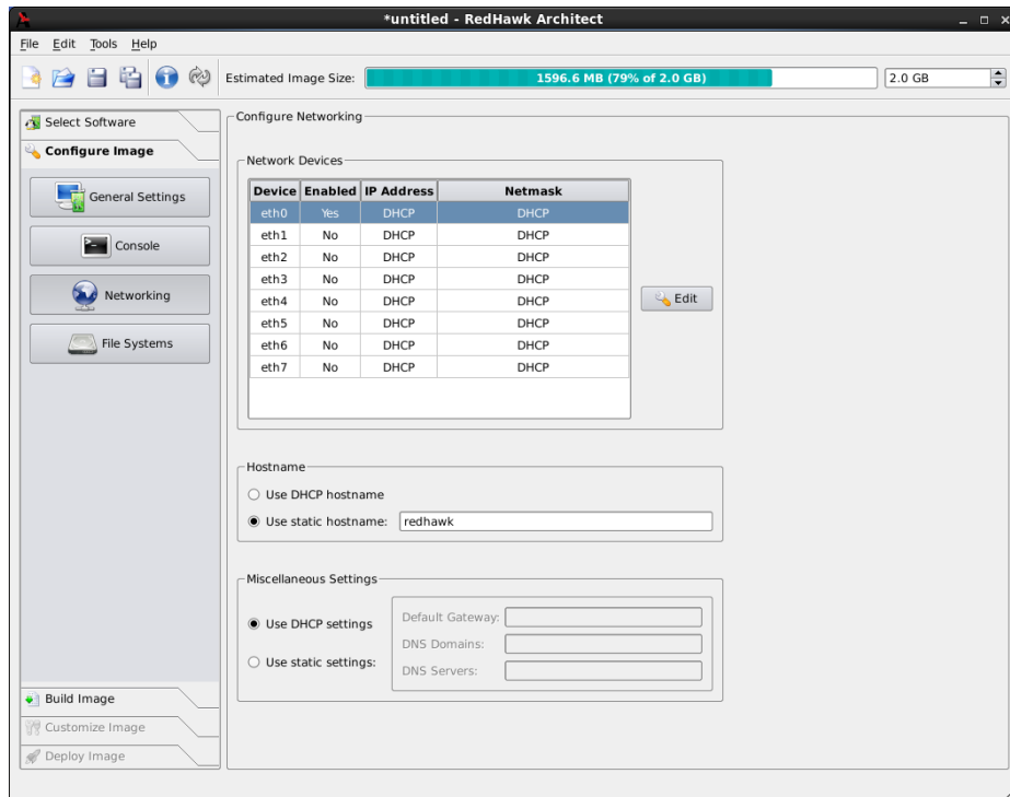
Figure 1-15 Network Configuration Page
