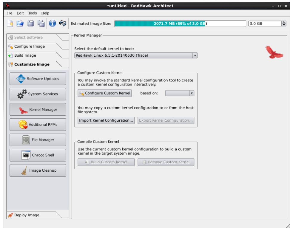
Figure 1-35 Kernel Manager Page
