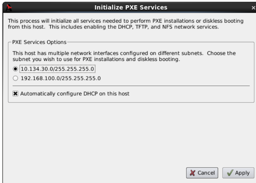
Figure 3-2 Initialize PXE Services Dialog
