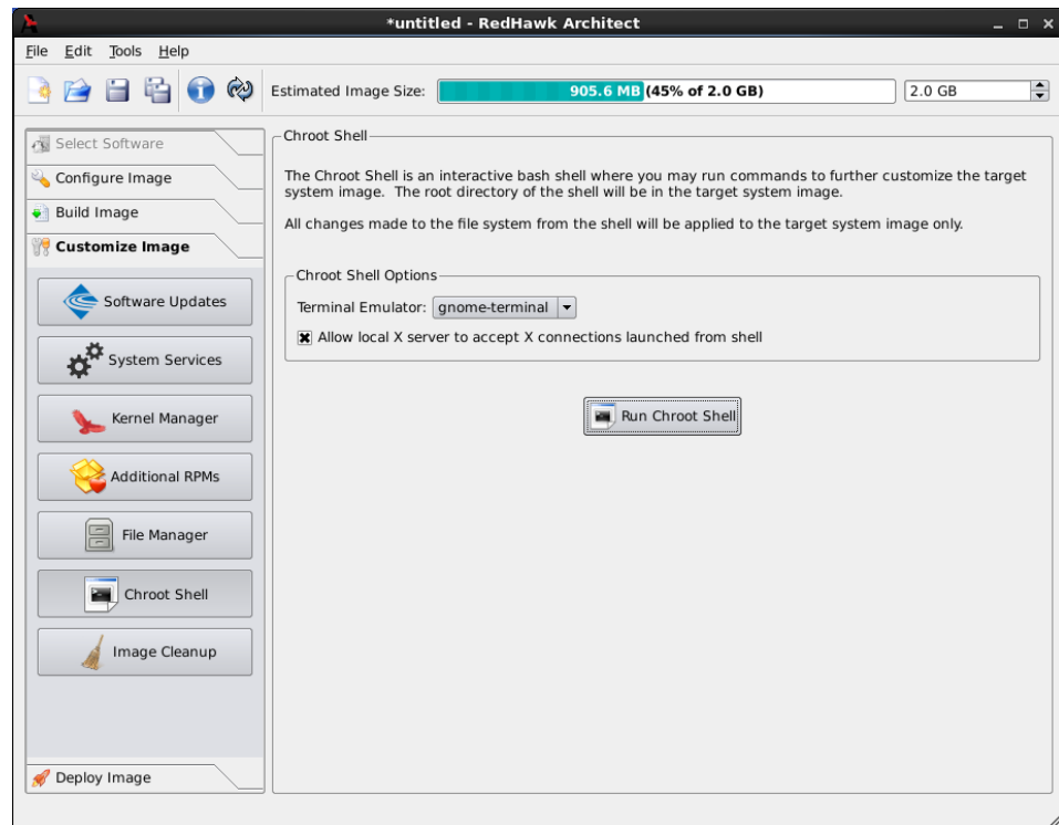
Figure 1-43 Chroot Shell Page
