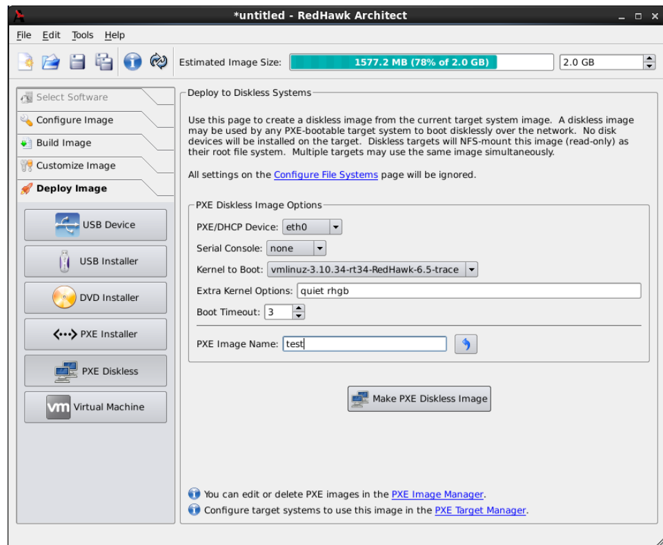
Figure 1-59 PXE Diskless Deployment Page
