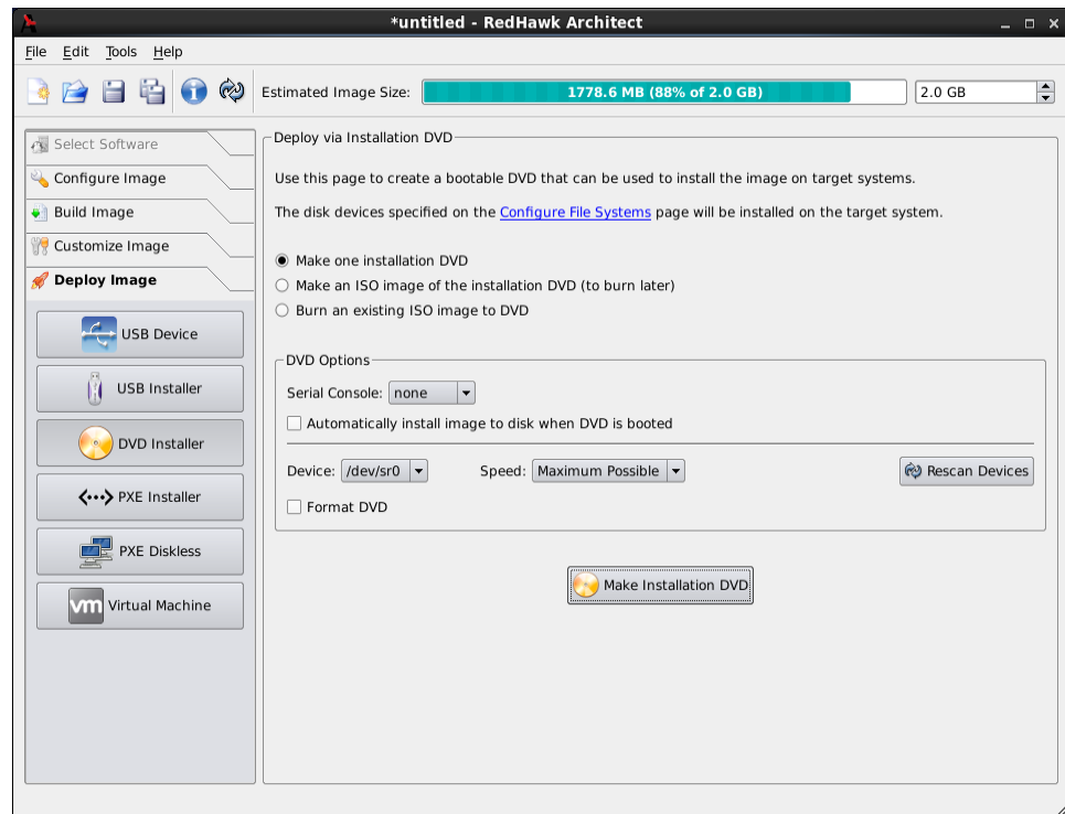
Figure 1-54 Deploy via Installation DVD Page
