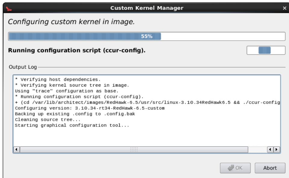
Figure 1-36 Custom Kernel Dialog
