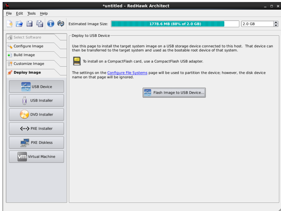
Figure 1-46 Deploy to USB Device Page
