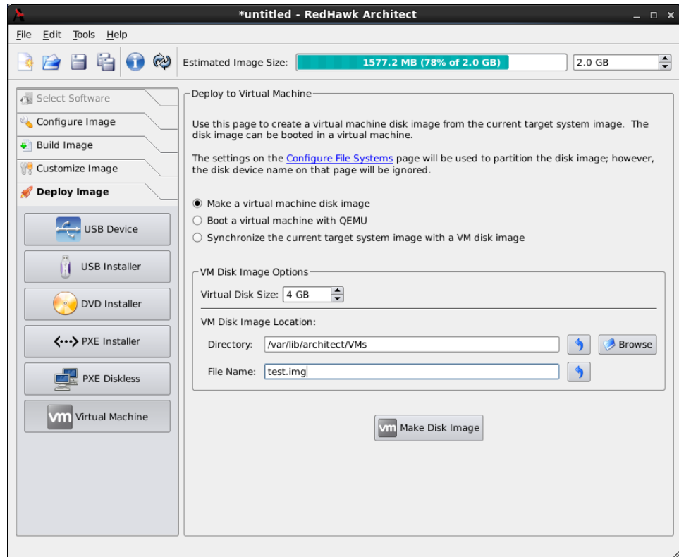
Figure 1-62 Deploy to Virtual Machine Page
