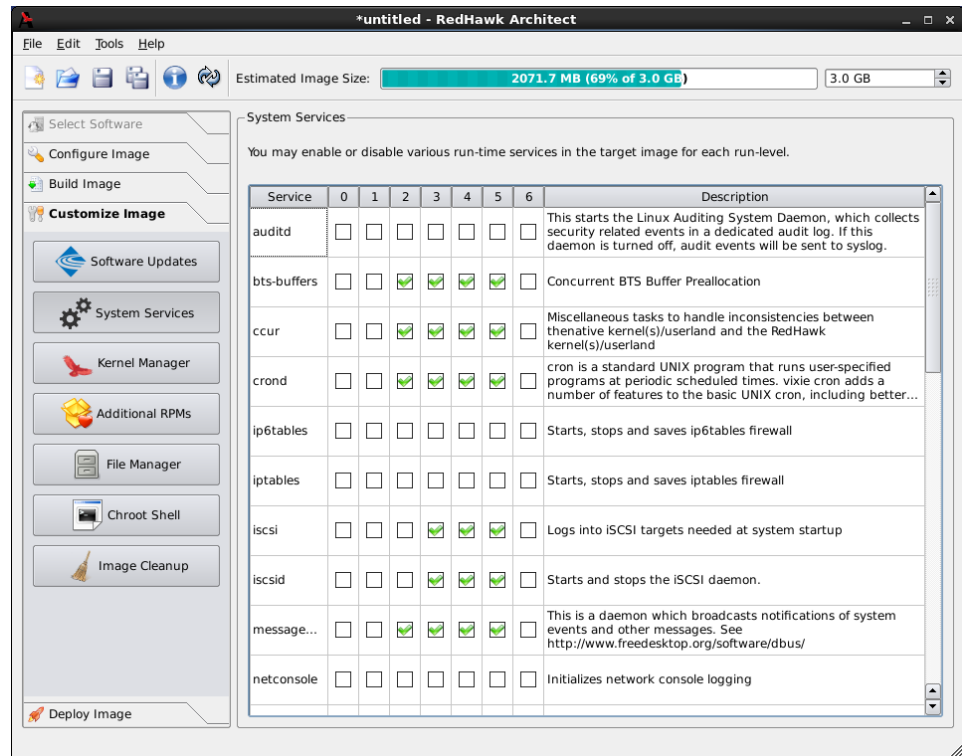
Figure 1-34 System Services Page
