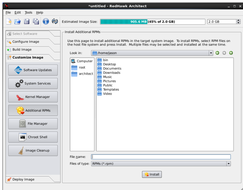
Figure 1-41 Install Additional RPMs Page
