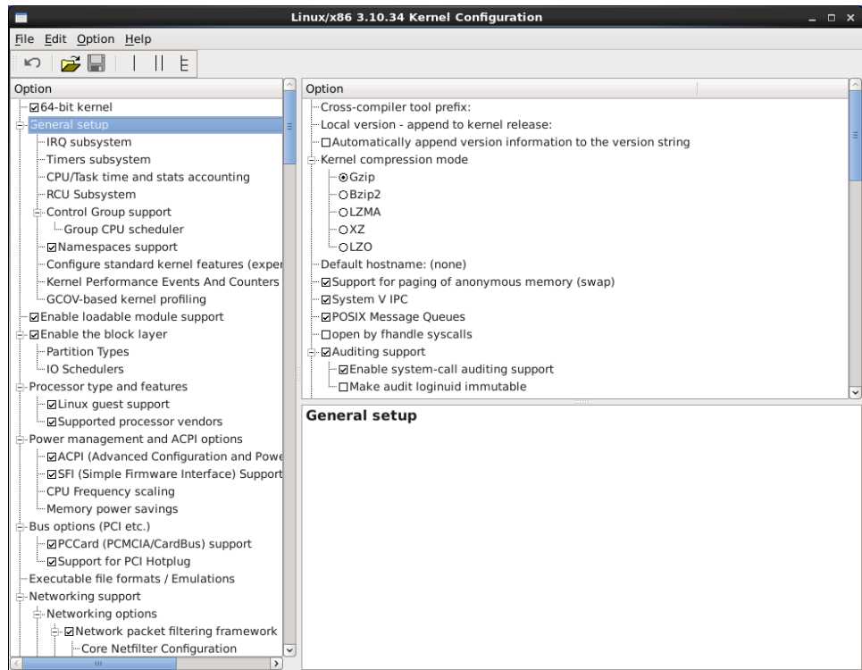
Figure 1-37 Linux Kernel Configuration Dialog
